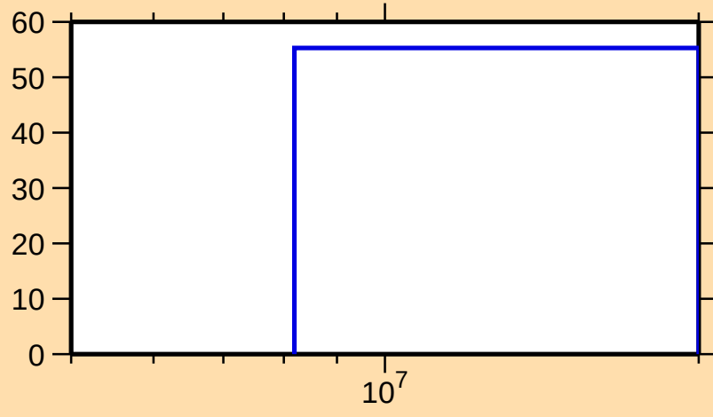
\Delta\sigma/\sigma vs. E for ^{156}\text{Nd}(n,n\text{cont.})
