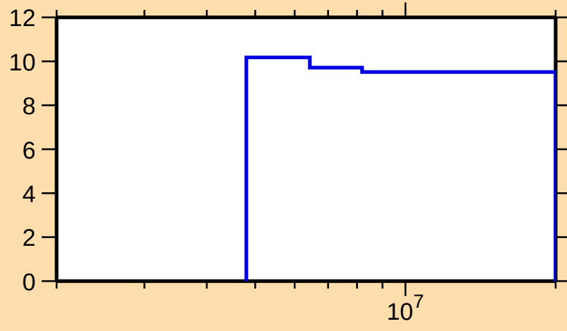
\Delta\sigma/\sigma vs. E for ^{156}\text{Nd}(n,\text{nonel.})
