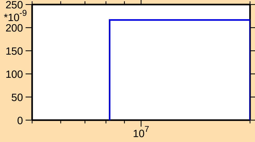
\sigma vs. E for ^{156}\text{Nd}(n,np)
