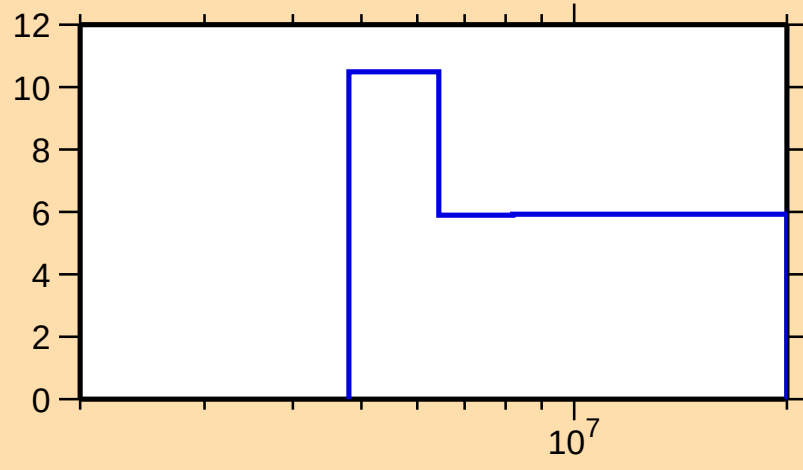
\Delta\sigma/\sigma vs. E for ^{156}\text{Nd}(n,\text{tot.})
