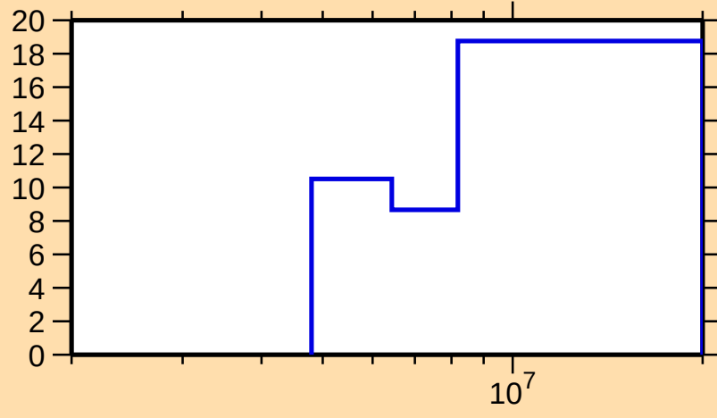
\Delta\sigma/\sigma vs. E for ^{156}\text{Nd}(n,2n)
