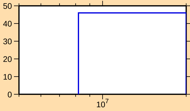
\Delta\sigma/\sigma vs. E for ^{156}\text{Nd}(n,\text{inel.})
