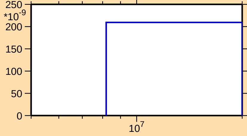
\sigma vs. E for ^{156}\text{Nd}(n,n\alpha)
