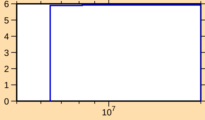
\Delta\sigma/\sigma vs. E for ^{156}\text{Nd}(n,\text{tot.})
