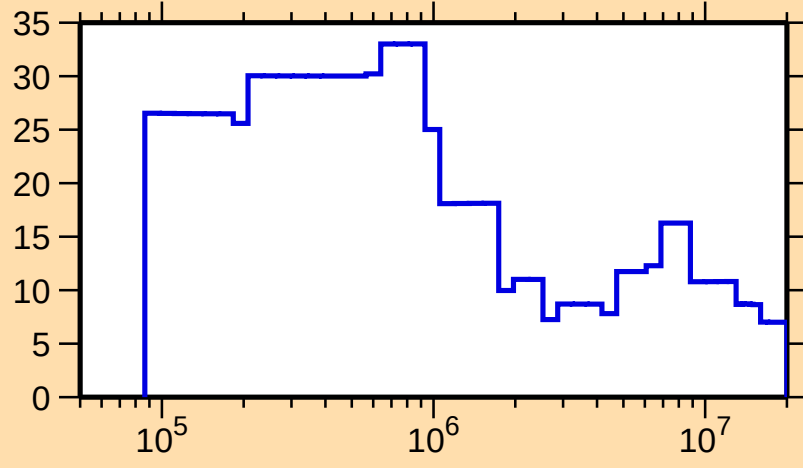
\Delta\sigma/\sigma vs. E for ^{286}\text{Po}
