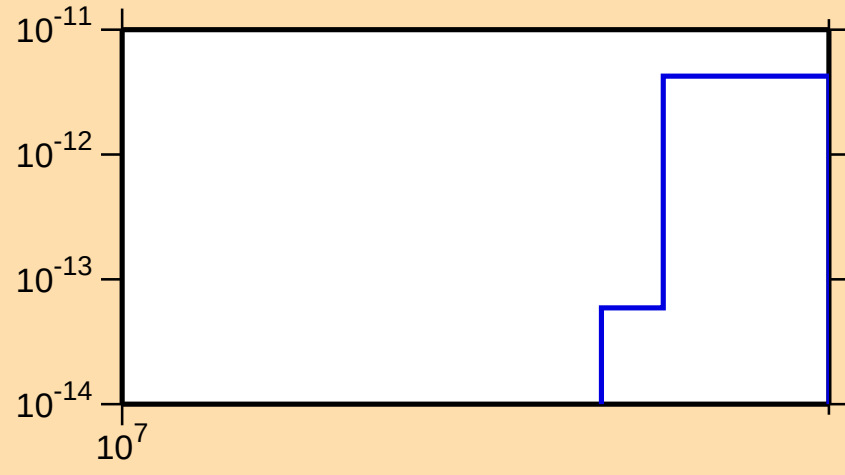
\sigma vs. E for ^{256}\text{No}(\text{mt } 34)
