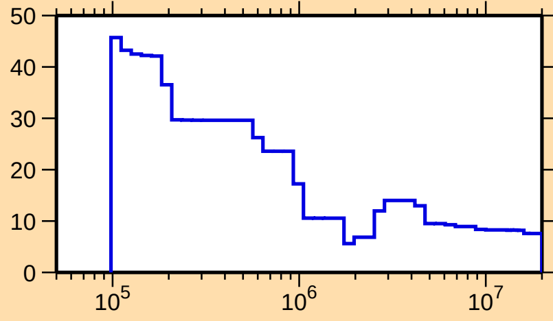
\Delta\sigma/\sigma vs. E for ^{256}\text{No}(n,n\text{onel.})
