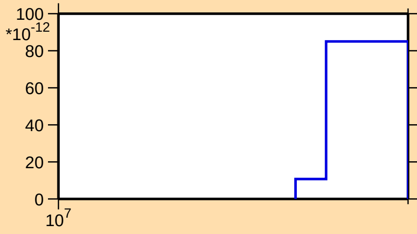
\sigma vs. E for ^{256}\text{No}(n,3n\alpha)
