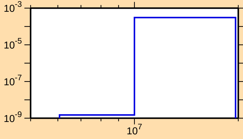
\sigma vs. E for ^{256}\text{No}(n,np)
