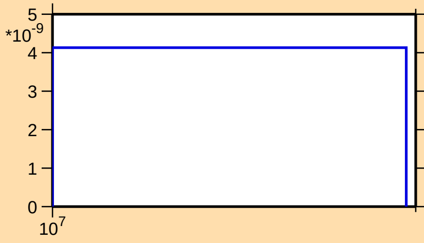
\sigma vs. E for ^{256}\text{No}(n,2np)
