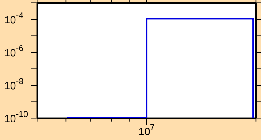
\sigma vs. E for ^{256}\text{No}(n,t)
