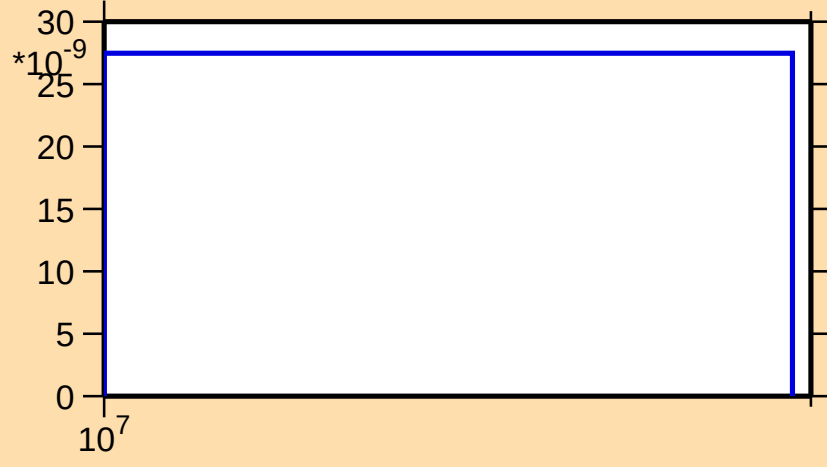
\sigma vs. E for ^{256}\text{No}(n,nt)
