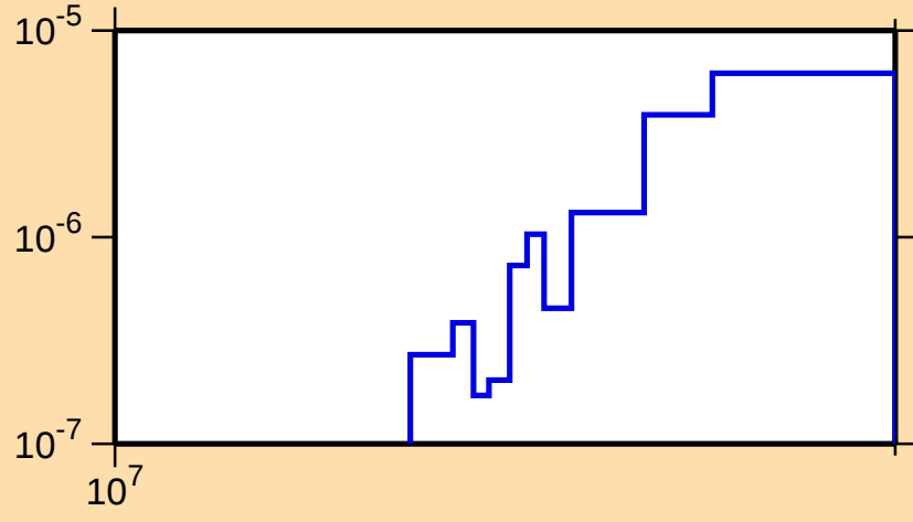
\sigma vs. E for ^{257}\text{No}(n,p\alpha)
