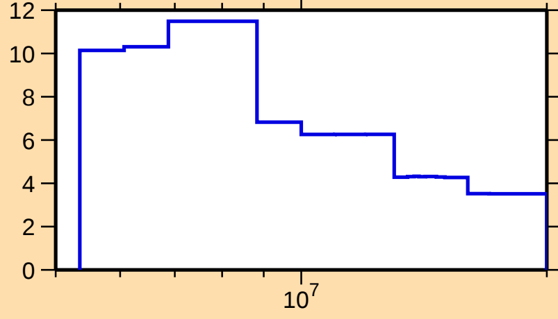
\Delta\sigma/\sigma vs. E for ^{257}\text{No}(n,\text{tot.})
