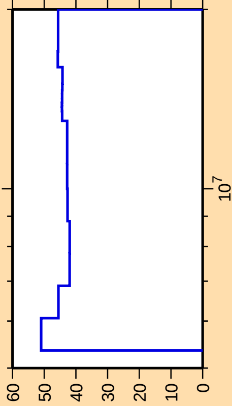
\Delta\sigma/\sigma vs. E for ^{257}\text{No}(n,\alpha)
