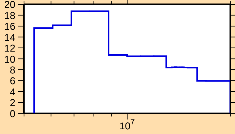
\Delta\sigma/\sigma vs. E for ^{257}\text{No}(n,\text{el.})
