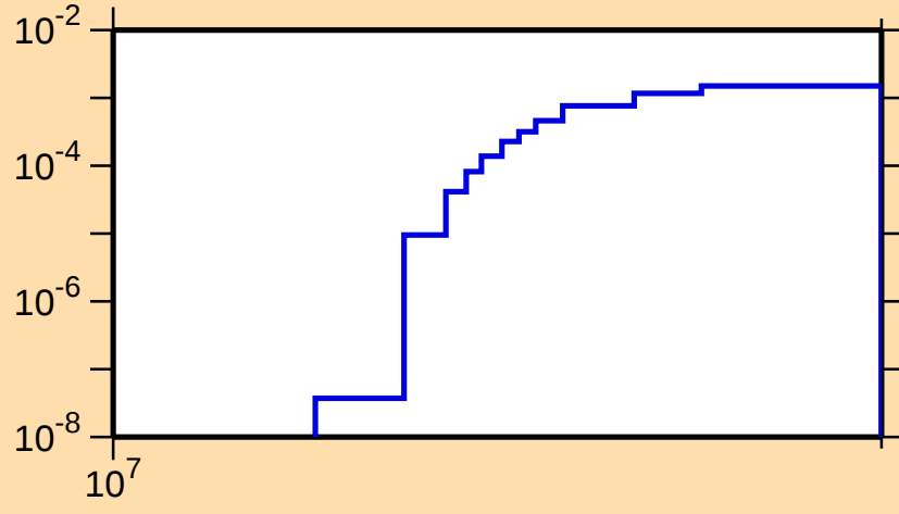
\sigma vs. E for ^{257}\text{No}(n,3n)
