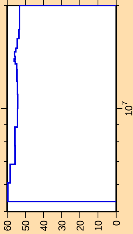
\Delta\sigma/\sigma vs. E for ^{257}\text{No}(n,n_1)
