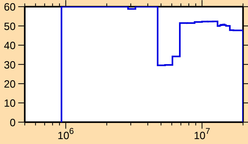
\Delta\sigma/\sigma vs. E for ^{257}\text{No}(n,\gamma)
