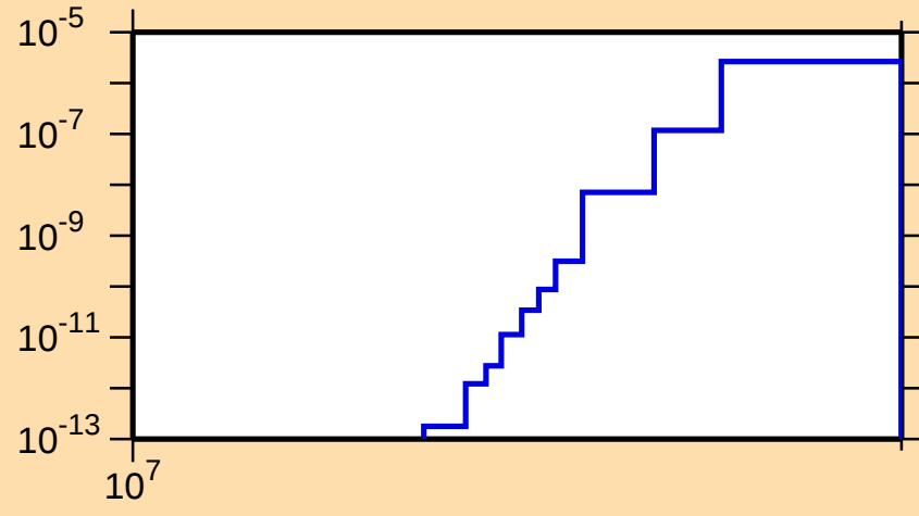
\sigma vs. E for ^{257}\text{No}(n,nt)
