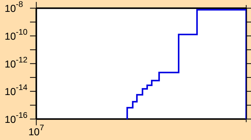
\sigma vs. E for ^{257}\text{No}(n,3n\alpha)
