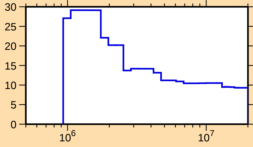
\Delta\sigma/\sigma vs. E for ^{257}\text{No}(n,\text{nonel.})
