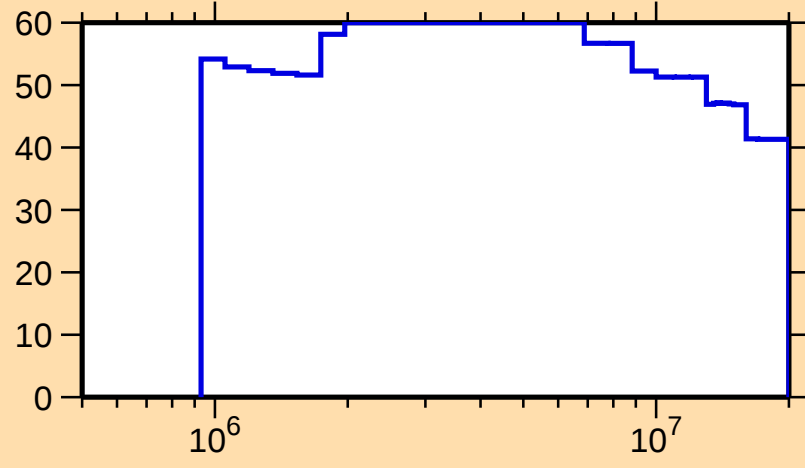
\Delta\sigma/\sigma vs. E for ^{257}\text{No}(n,f)
