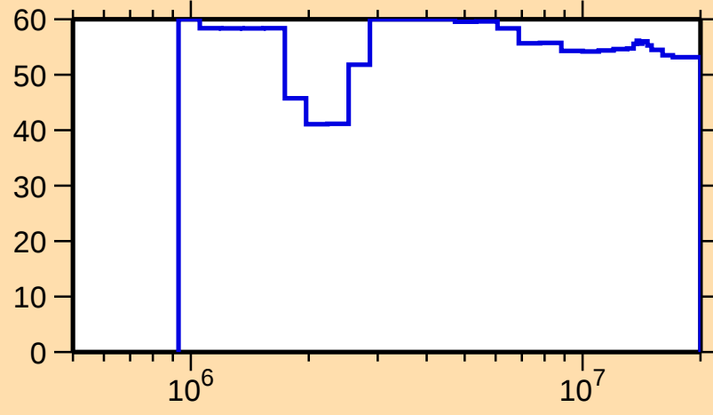
\Delta\sigma/\sigma vs. E for ^{257}\text{No}(n,n_1)
