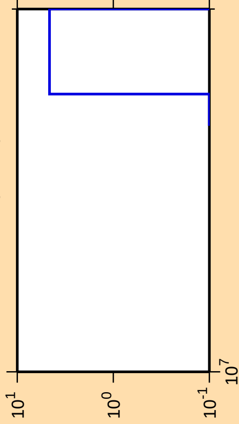
\Delta\sigma/\sigma vs. E for ^{257}\text{No}(\text{mt } 34)
