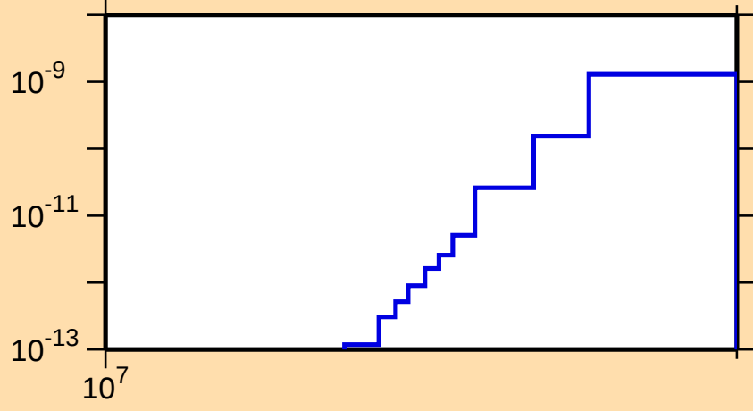
\sigma vs. E for ^{257}\text{No}(n,\text{He3})
