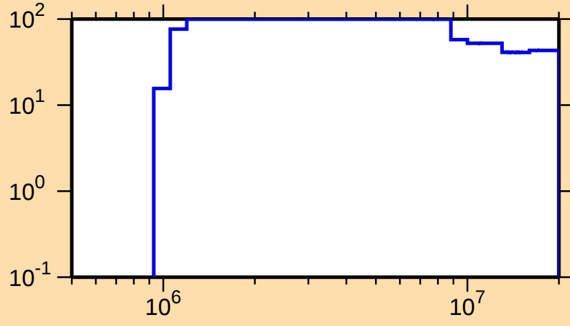
\Delta\sigma/\sigma vs. E for ^{257}\text{No}(n,p)
