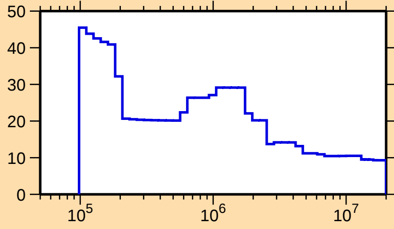
\Delta\sigma/\sigma vs. E for ^{257}\text{No}(n,n\text{onel.})
