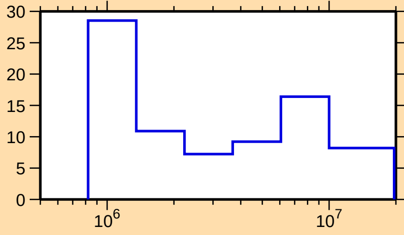
\Delta\sigma/\sigma vs. E for ^{257}\text{No}(n,\text{el.})
