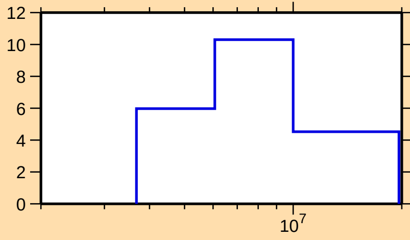
\Delta\sigma/\sigma vs. E for ^{257}\text{No}(n,\text{tot.})
