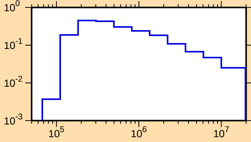
\sigma vs. E for ^{257}\text{No}(n,n_1)
