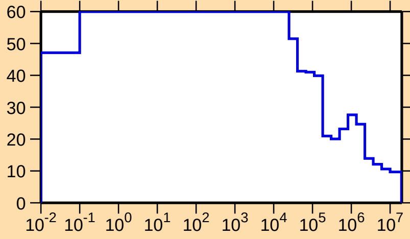
\Delta\sigma/\sigma vs. E for ^{257}\text{No}(n,\text{nonel.})
