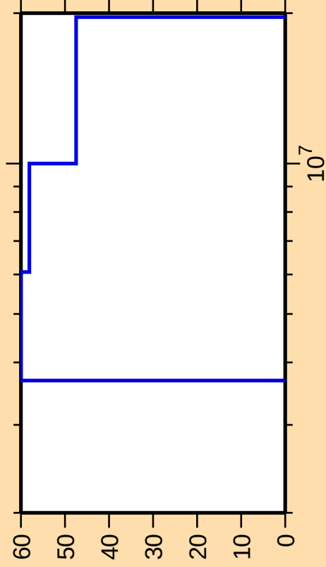
\Delta\sigma/\sigma vs. E for ^{257}\text{No}(n,f)
