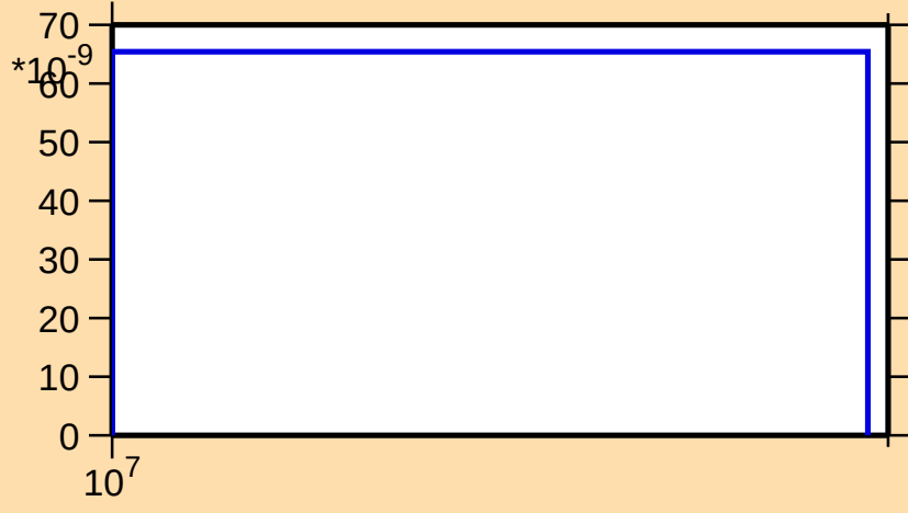
\sigma vs. E for ^{257}\text{No}(n,\text{nd})
