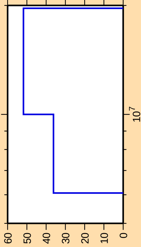
\Delta\sigma/\sigma vs. E for ^{257}\text{No}(n,t)
