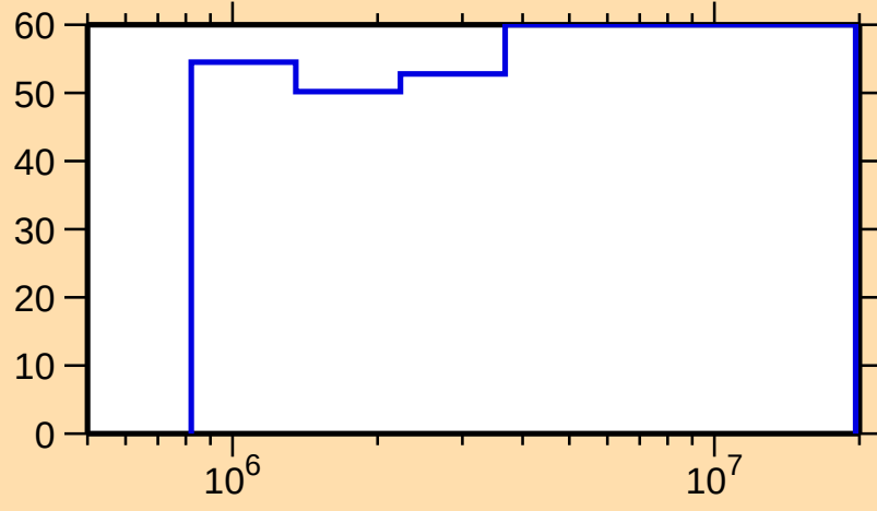
\Delta\sigma/\sigma vs. E for ^{257}\text{No}(n,n\text{cont.})
