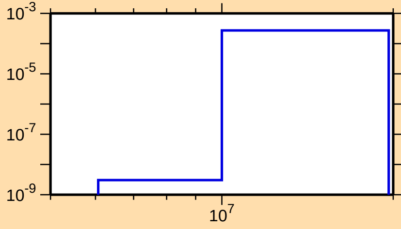
\sigma vs. E for ^{257}\text{No}(n,np)
