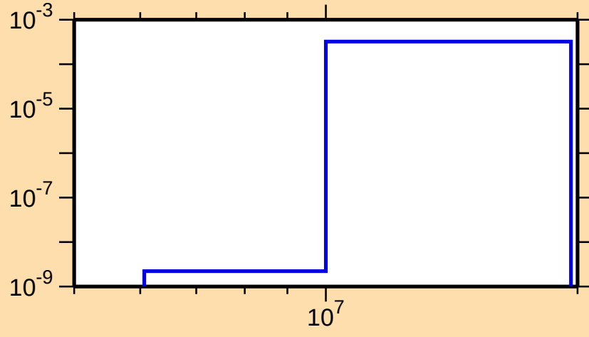
\sigma vs. E for ^{257}\text{No}(n,d)
