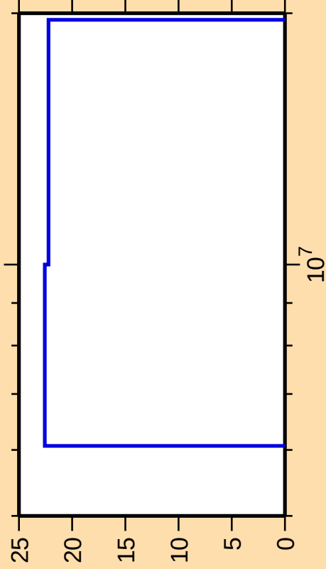
\Delta\sigma/\sigma vs. E for ^{257}\text{No}(n,d)
