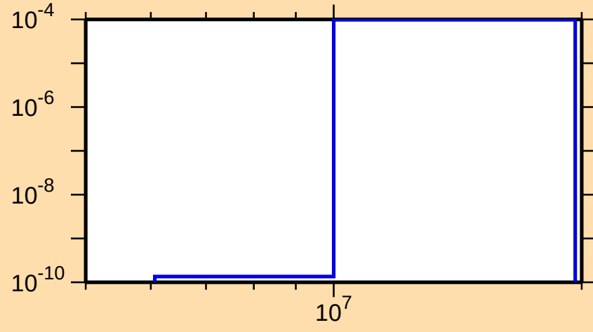
\sigma vs. E for ^{257}\text{No}(n,t)
