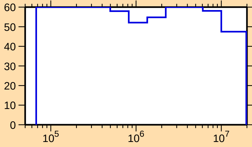
\Delta\sigma/\sigma vs. E for ^{257}\text{No}(n,f)
