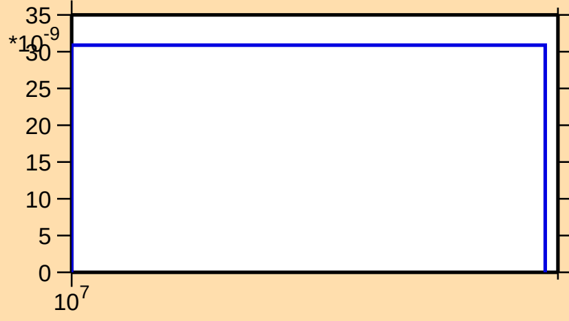
\sigma vs. E for ^{257}\text{No}(n,\text{nt})
