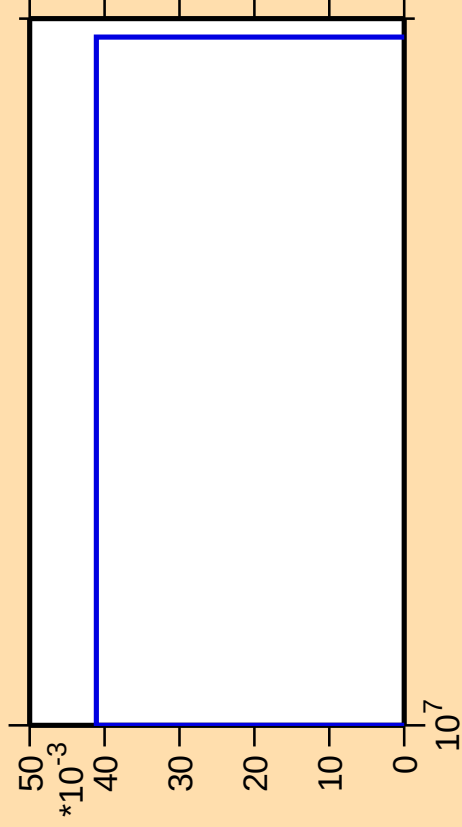
\Delta\sigma/\sigma vs. E for ^{257}\text{No}(\text{mt } 34)
