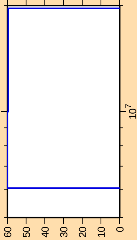
\Delta\sigma/\sigma vs. E for ^{257}\text{No}(n,np)
