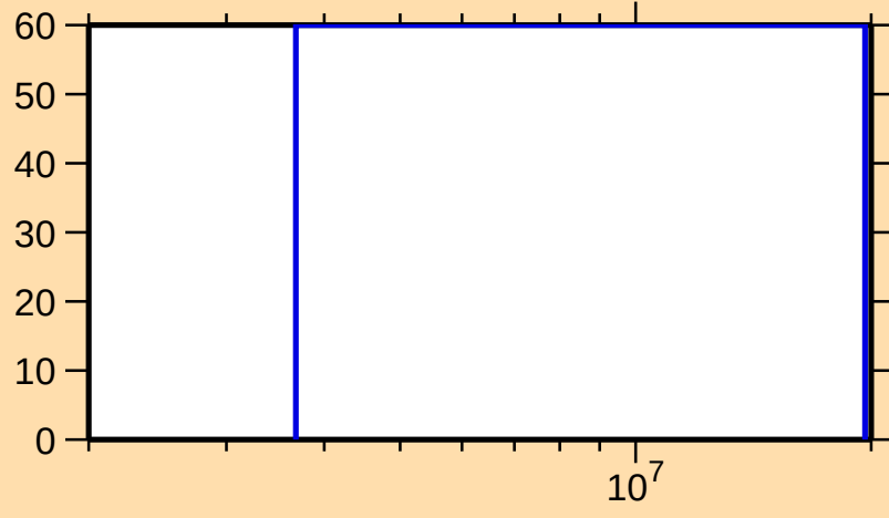
\Delta\sigma/\sigma vs. E for ^{257}\text{No}(n,2n)
