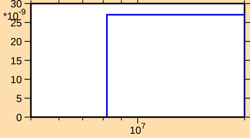
\sigma vs. E for ^{257}\text{No}(n,nt)
