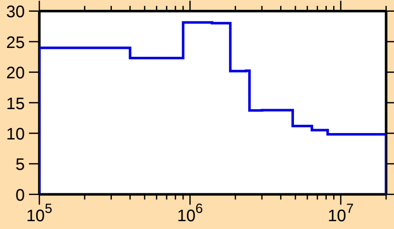
\Delta\sigma/\sigma vs. E for ^{257}\text{No}(n,n\text{onel.})
