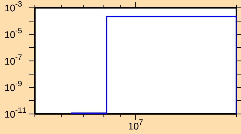
\sigma vs. E for ^{257}\text{No}(n,np)
