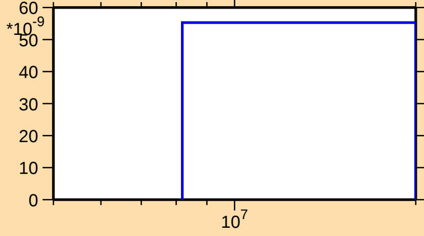
\sigma vs. E for ^{257}\text{No}(n,\text{nd})
