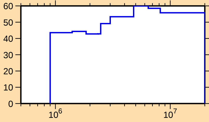
\Delta\sigma/\sigma vs. E for ^{257}\text{No}(n,\text{inel.})
