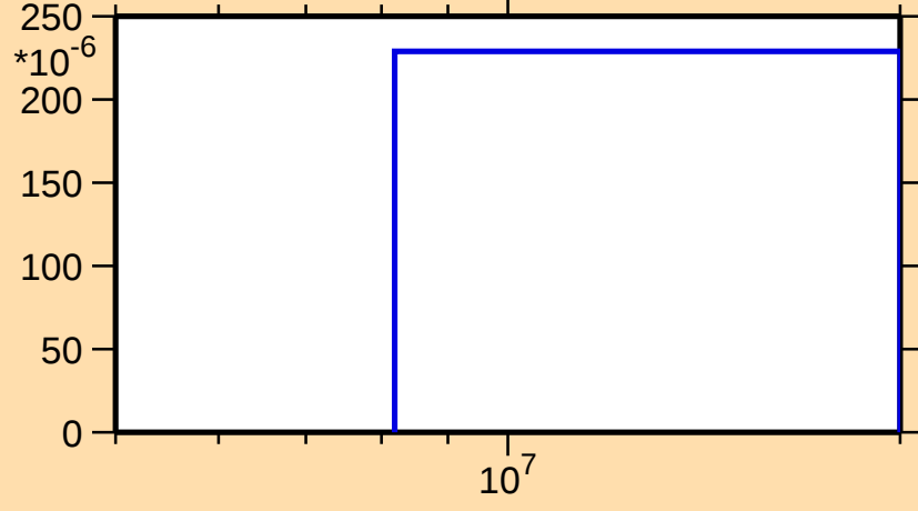
\sigma vs. E for ^{257}\text{No}(n,3n)
