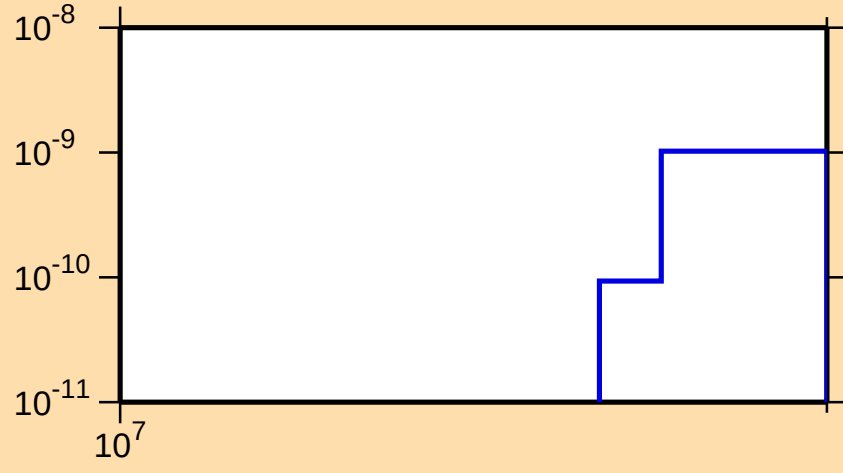
\sigma vs. E for ^{261}\text{No}(n,\text{He3})
