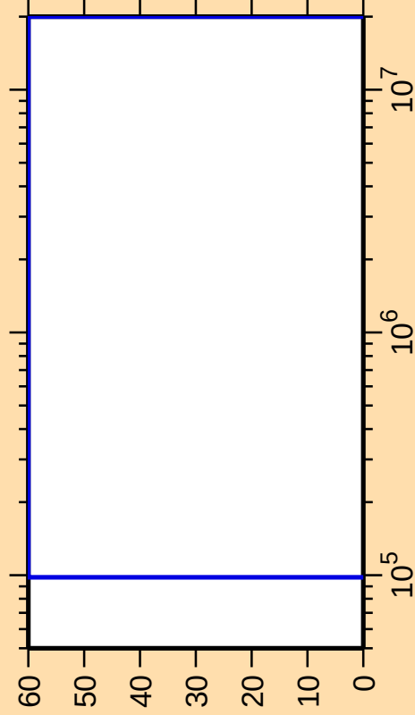
\Delta\sigma/\sigma vs. E for ^{261}\text{No}(n,\text{ncont.})
