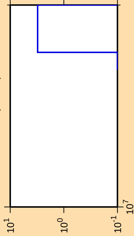
\Delta\sigma/\sigma vs. E for ^{261}\text{No}(\text{mt } 34)
