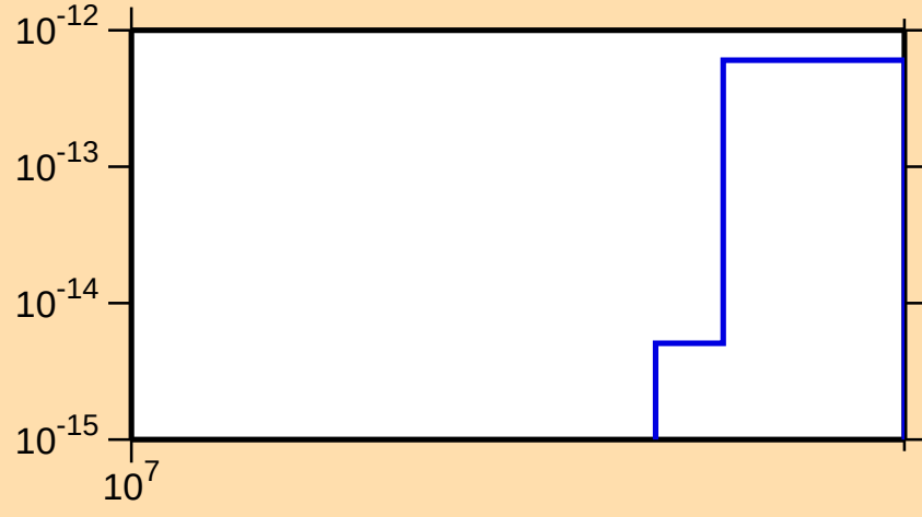
\sigma vs. E for ^{261}\text{No}(\text{mt } 34)
