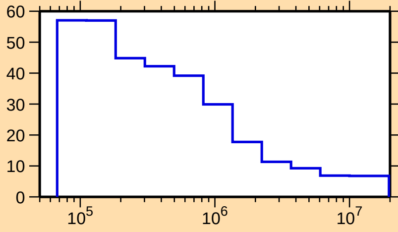
\Delta\sigma/\sigma vs. E for ^{261}\text{No}(n,\text{nonel.})
