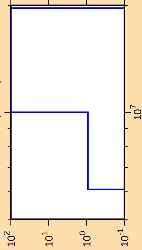
\Delta\sigma/\sigma vs. E for ^{261}\text{No}(n,2n\alpha)
