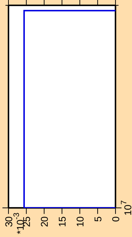
\Delta\sigma/\sigma vs. E for ^{261}\text{No}(\text{mt } 34)
