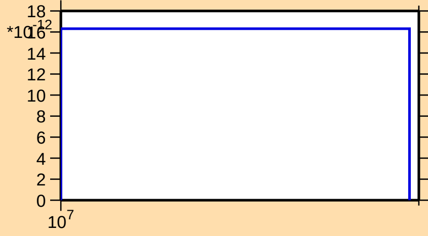
\sigma vs. E for ^{261}\text{No}(n,\text{He3})
