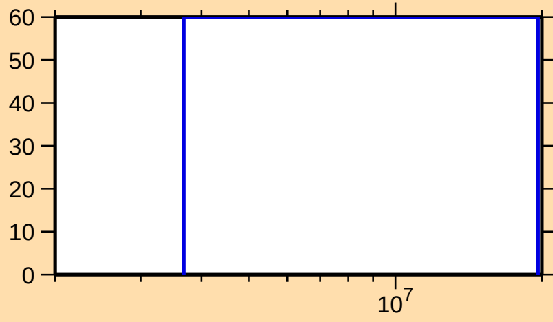
\Delta\sigma/\sigma vs. E for ^{261}\text{No}(n,2n)
