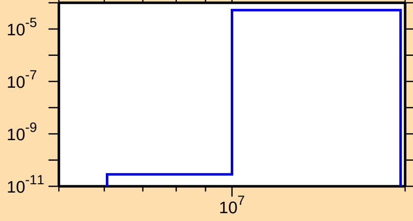
\sigma vs. E for ^{261}\text{No}(n,t)
