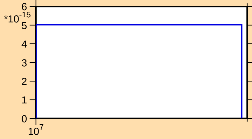
\sigma vs. E for ^{261}\text{No}(n,3n\alpha)
