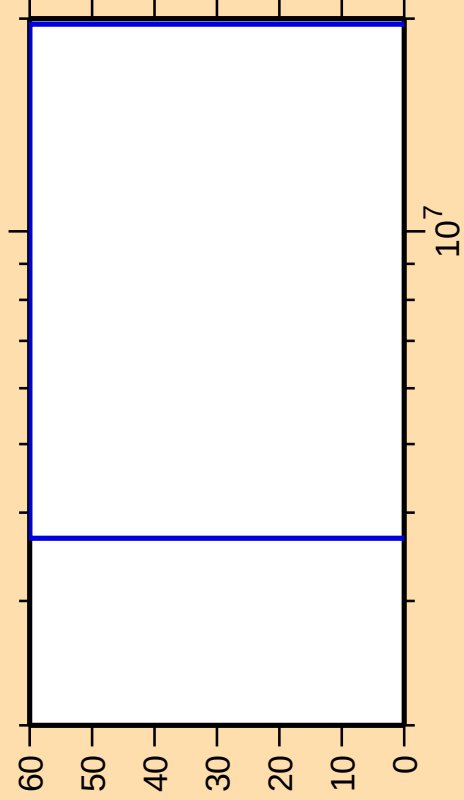
\Delta\sigma/\sigma vs. E for ^{261}\text{No}(n,\gamma)
