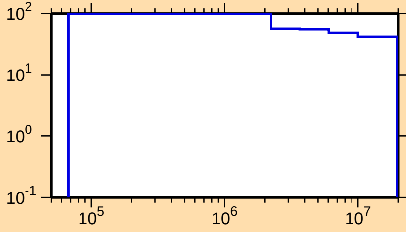
\Delta\sigma/\sigma vs. E for ^{261}\text{No}(n,n_1)
