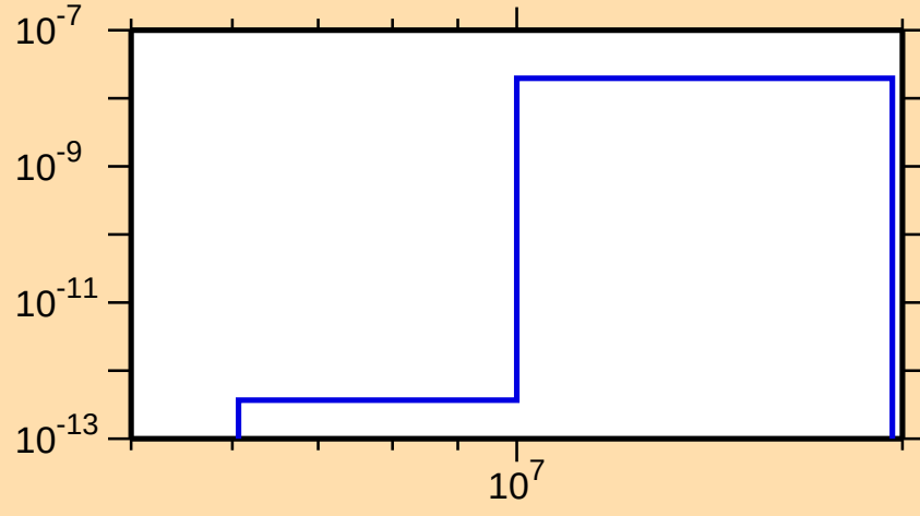
\sigma vs. E for ^{261}\text{No}(n,2n\alpha)
