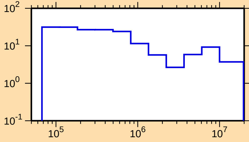
\Delta\sigma/\sigma vs. E for ^{261}\text{No}(n,\text{tot.})
