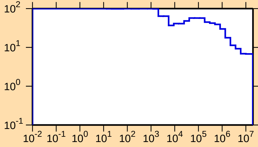
\Delta\sigma/\sigma vs. E for ^{261}\text{No}(n,\text{nonel.})
