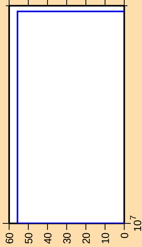
\Delta\sigma/\sigma vs. E for ^{261}\text{No}(n,\text{He3})
