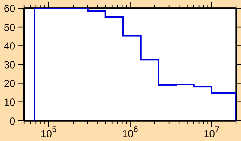
\Delta\sigma/\sigma vs. E for ^{261}\text{No}(n,f)
