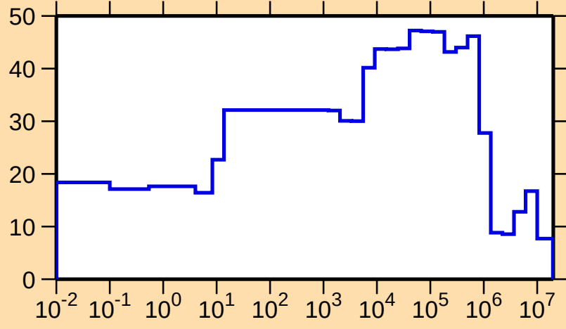
\Delta\sigma/\sigma vs. E for ^{261}\text{No}(n,\text{el.})
