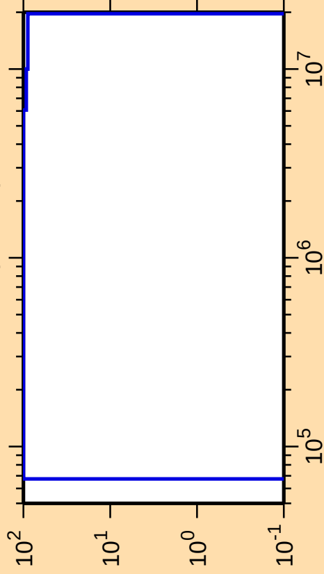
\Delta\sigma/\sigma vs. E for ^{261}\text{No}(n,\text{inel.})
