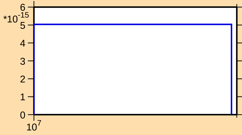
\sigma vs. E for ^{261}\text{No}(\text{mt } 34)
