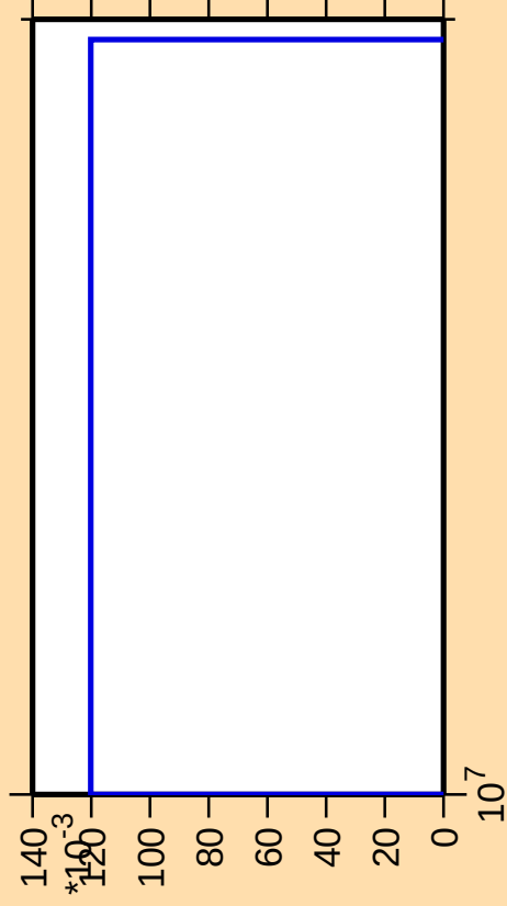
\Delta\sigma/\sigma vs. E for ^{261}\text{No}(n,3n\alpha)
