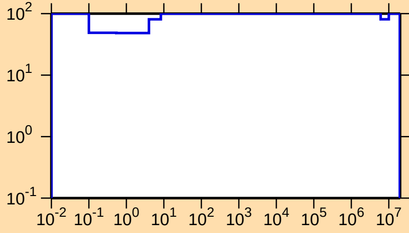
\Delta\sigma/\sigma vs. E for ^{261}\text{No}(n,\gamma)
