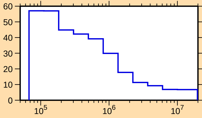
\Delta\sigma/\sigma vs. E for ^{261}\text{No}(n,n\text{onel.})
