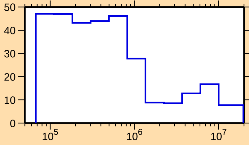
\Delta\sigma/\sigma vs. E for ^{261}\text{No}(n,\text{el.})
