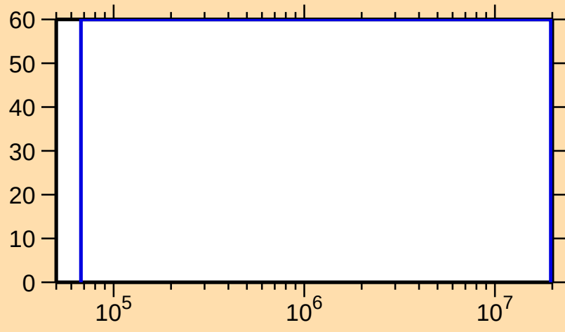
\Delta\sigma/\sigma vs. E for ^{261}\text{No}(n,n\text{cont.})
