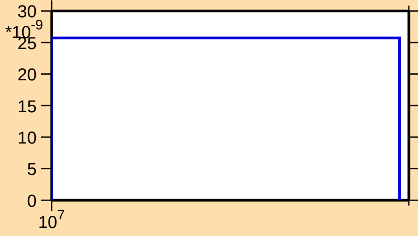
\sigma vs. E for ^{261}\text{No}(n,nt)
