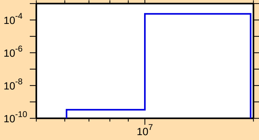
\sigma vs. E for ^{261}\text{No}(n,d)
