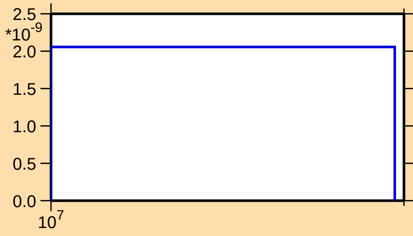
\sigma vs. E for ^{261}\text{No}(n,2np)
