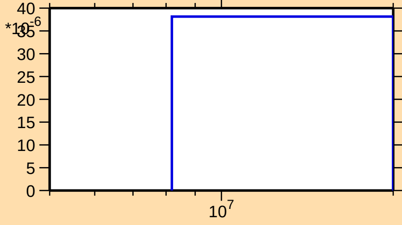
\sigma vs. E for ^{261}\text{No}(n,np)
