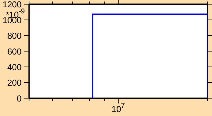
\sigma vs. E for ^{261}\text{No}(n,3n)
