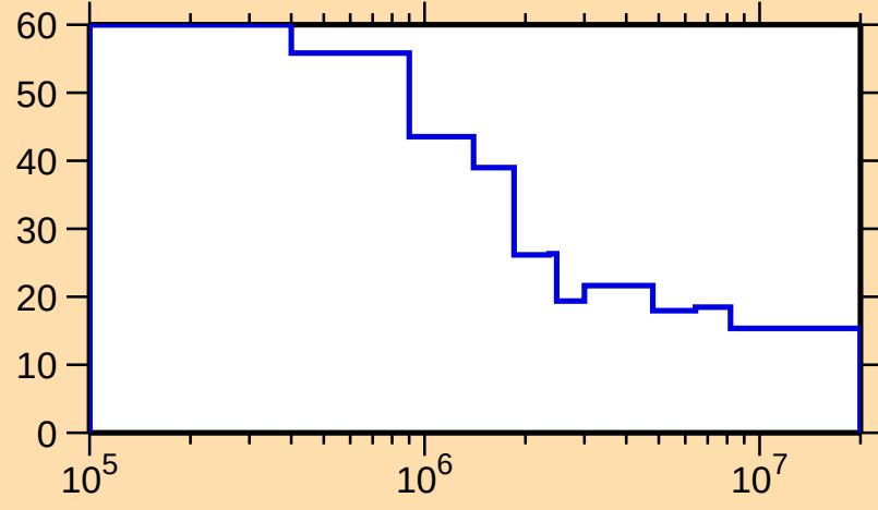
\Delta\sigma/\sigma vs. E for ^{261}\text{No}(n,f)
