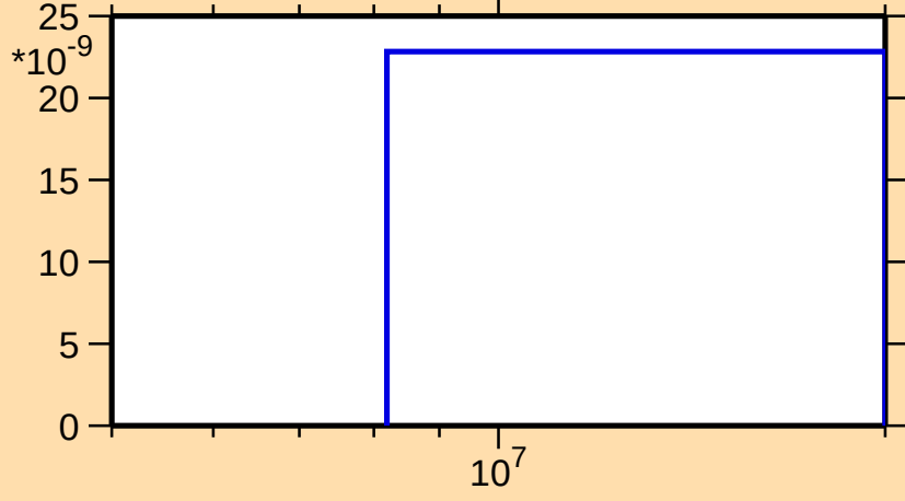
\sigma vs. E for ^{261}\text{No}(n,nt)
