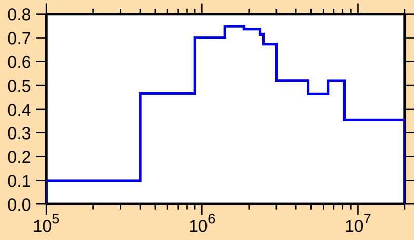
\sigma vs. E for ^{261}\text{No}(n,\text{inel.})
