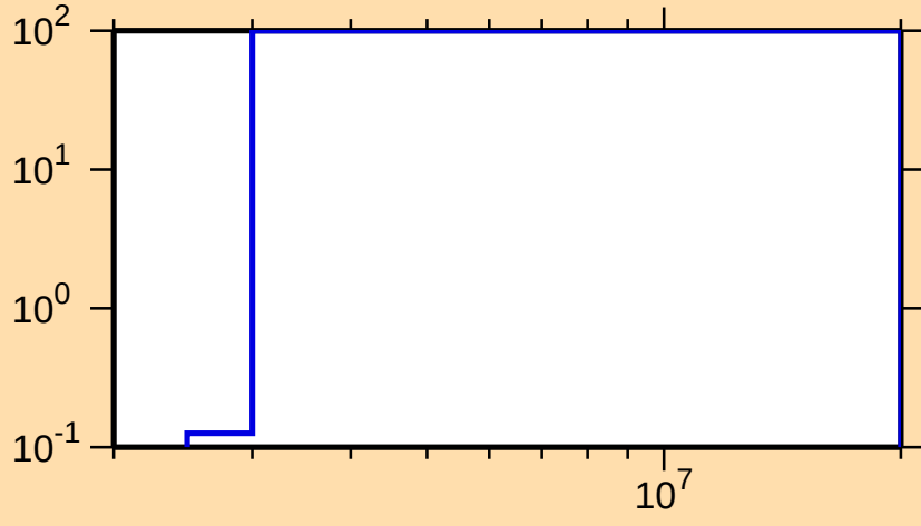
\Delta\sigma/\sigma vs. E for ^{261}\text{No}(n,p)
