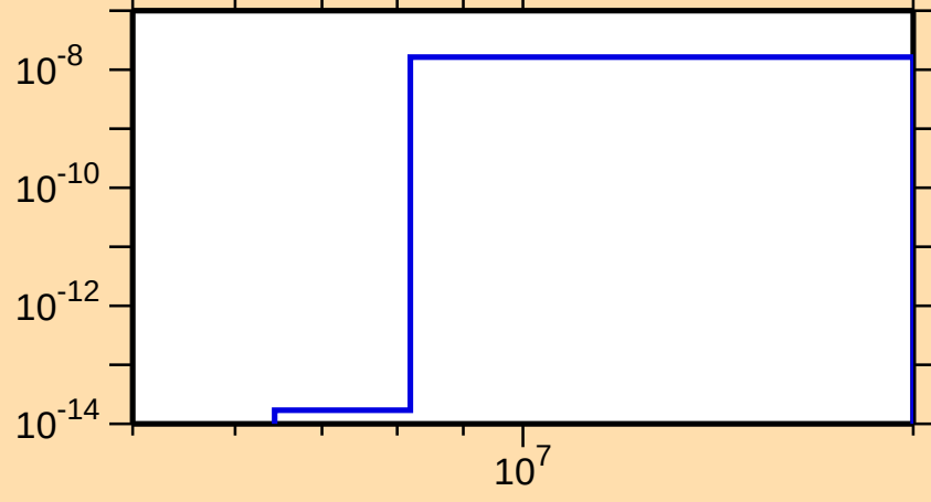
\sigma vs. E for ^{261}\text{No}(n,2n\alpha)
