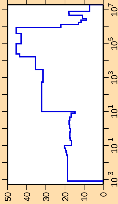
\Delta\sigma/\sigma vs. E for ^{261}\text{No}(n,\text{el.})
