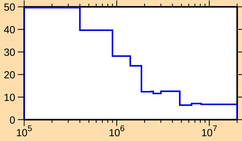
\Delta\sigma/\sigma vs. E for ^{261}\text{No}(n,n\text{nonel.})
