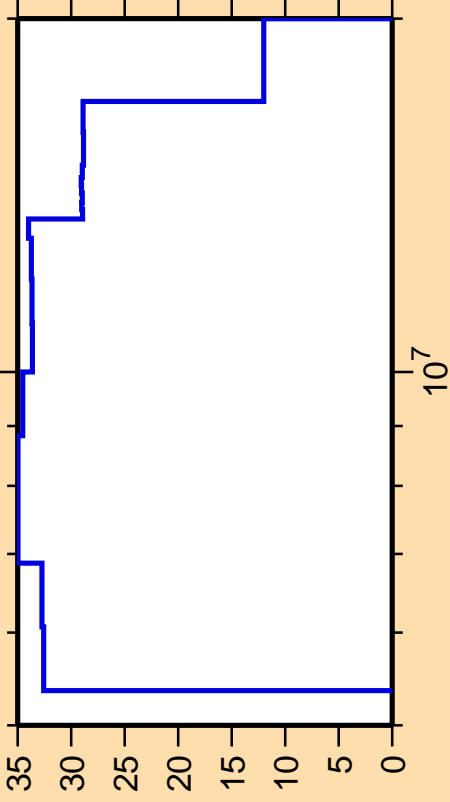
\Delta\sigma/\sigma vs. E for ^{14}\text{O}(n,n_1)
