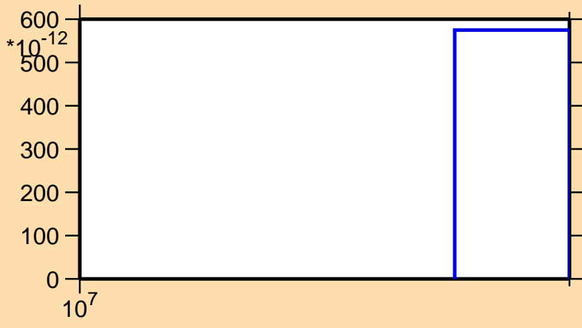
\sigma vs. E for ^{14}\text{O} (mt 34)
