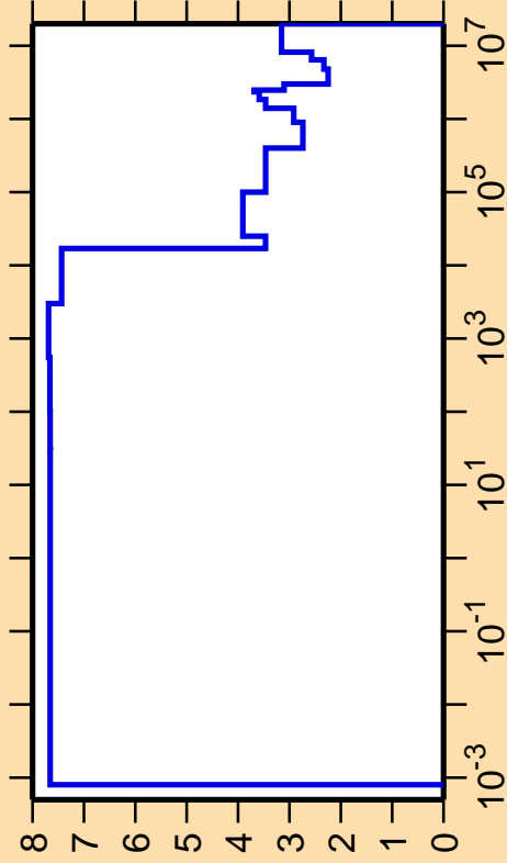
\Delta\sigma/\sigma vs. E for ^{14}\text{O}(n,\text{el.})
