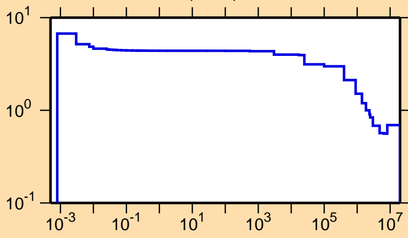
\sigma vs. E for ^{14}\text{O}(n,\text{el.})
