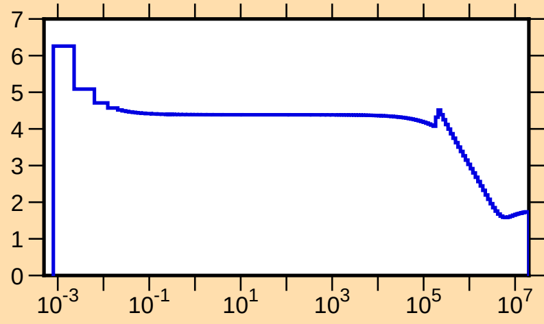
\sigma vs. E for ^{19}\text{O}(\text{n,tot.})
