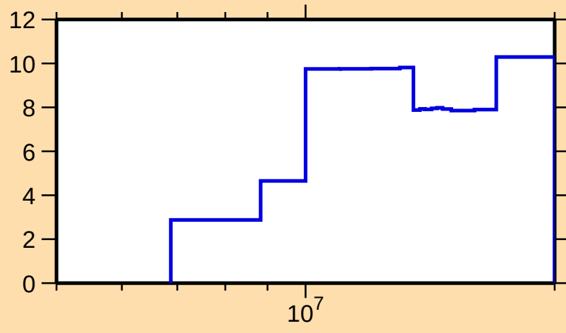
\Delta\sigma/\sigma vs. E for ^{19}\text{O}(\text{n,incl.})
