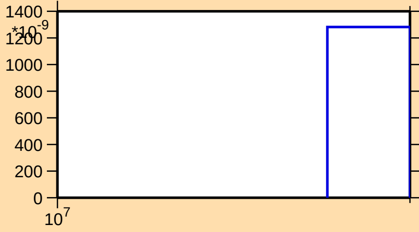
\sigma vs. E for ^{19}\text{O}(\text{n},\text{np})
