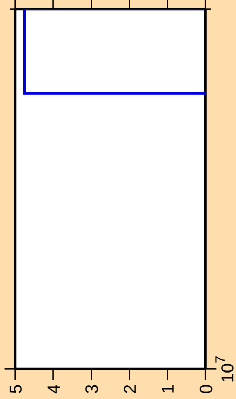
\Delta\sigma/\sigma vs. E for ^{19}\text{O}(n,3n\alpha)
