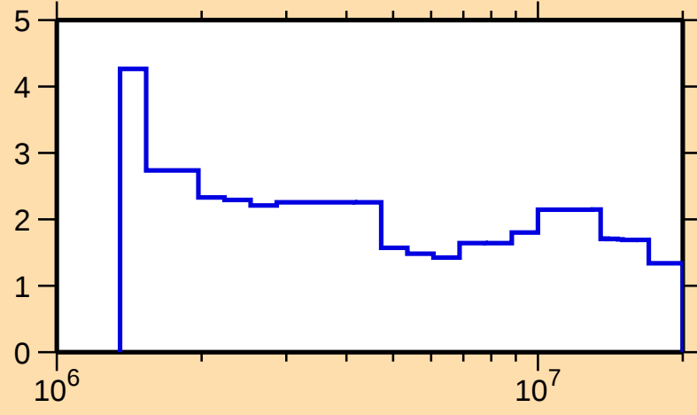
\Delta\sigma/\sigma vs. E for ^{21}\text{O}(n,\text{tot.})
