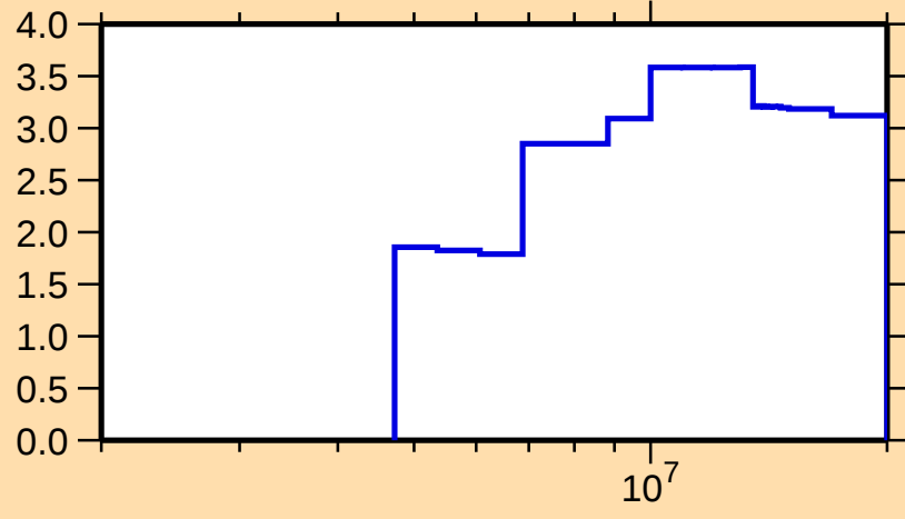
\Delta\sigma/\sigma vs. E for ^{21}\text{O}(\text{n},\text{el.})
