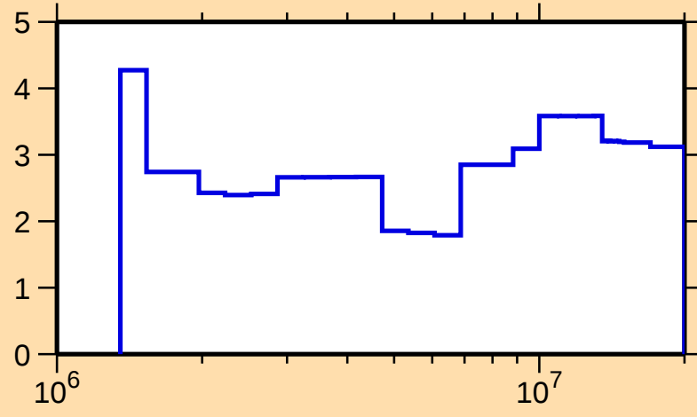
\Delta\sigma/\sigma vs. E for ^{21}\text{O}(n,\text{el.})
