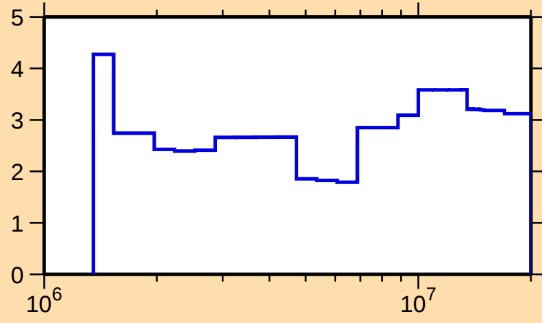
\Delta\sigma/\sigma vs. E for ^{21}\text{O}(\text{n,el.})
