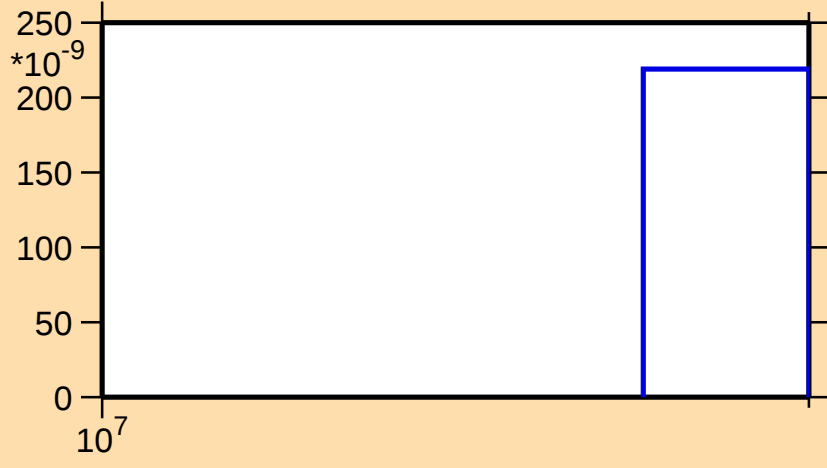
\sigma vs. E for ^{21}\text{O}(\text{n,p})
