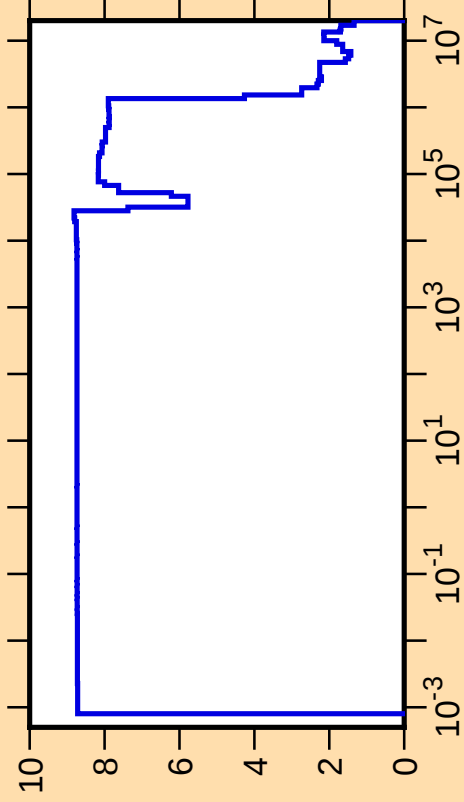
\Delta\sigma/\sigma vs. E for ^{21}\text{O}(\text{n,tot.})
