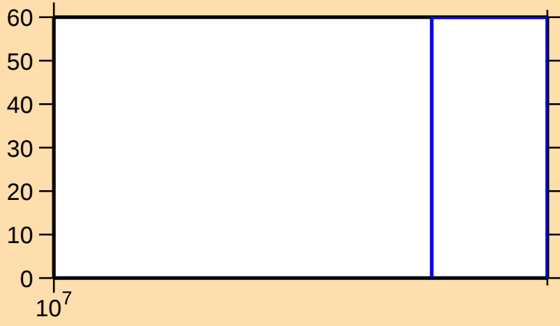
\Delta\sigma/\sigma vs. E for ^{21}\text{O}(n,\gamma)
