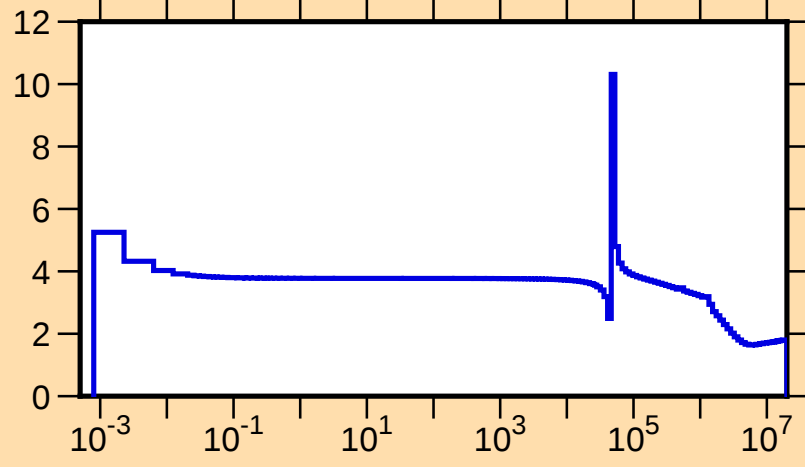
\sigma vs. E for ^{21}\text{O}(\text{n,tot.})
