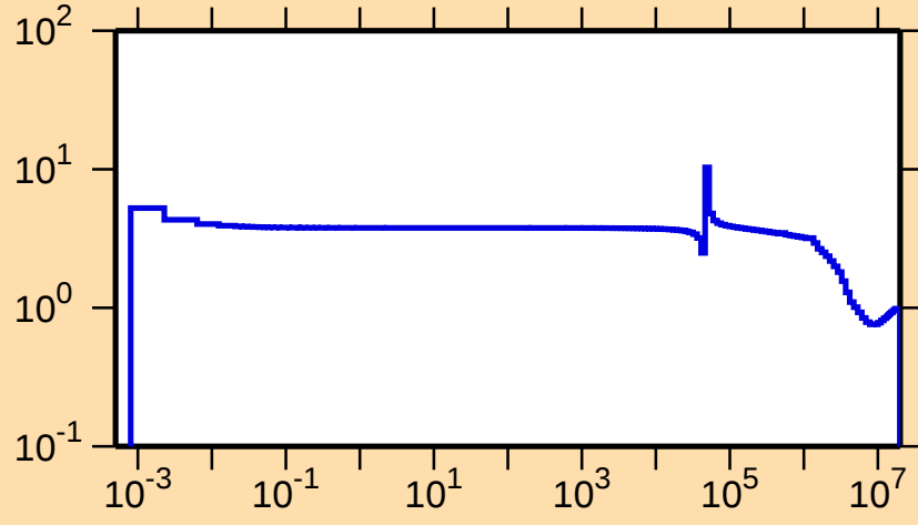
\sigma vs. E for ^{21}\text{O}(\text{n,el.})
