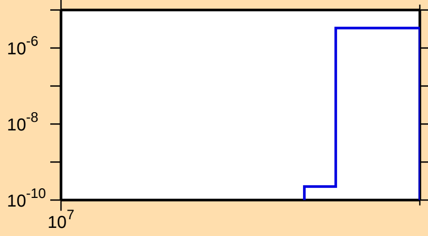
\sigma vs. E for ^{21}\text{O}(n,n\alpha)
