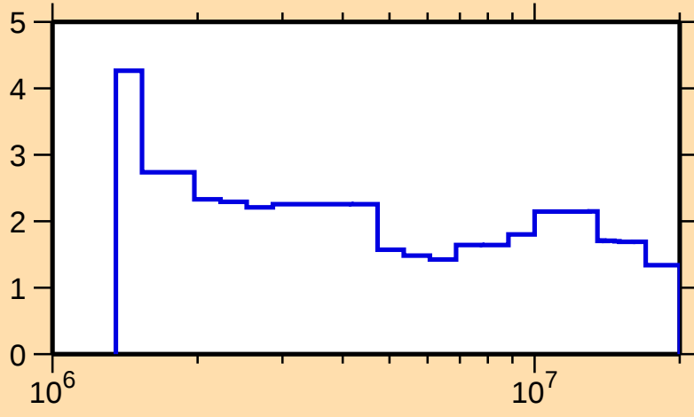
\Delta\sigma/\sigma vs. E for ^{21}\text{O}(\text{n,tot.})
