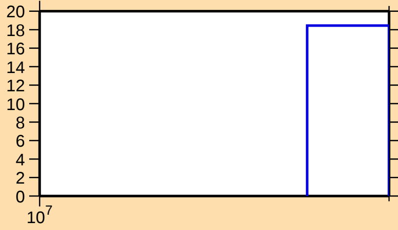
\Delta\sigma/\sigma vs. E for ^{21}\text{O}(\text{n,n}_1)
