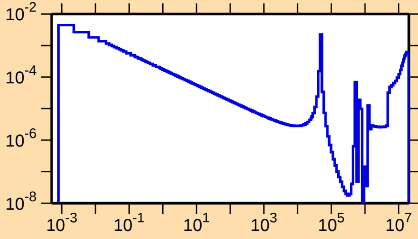
\sigma vs. E for ^{21}\text{O}(n,\gamma)
