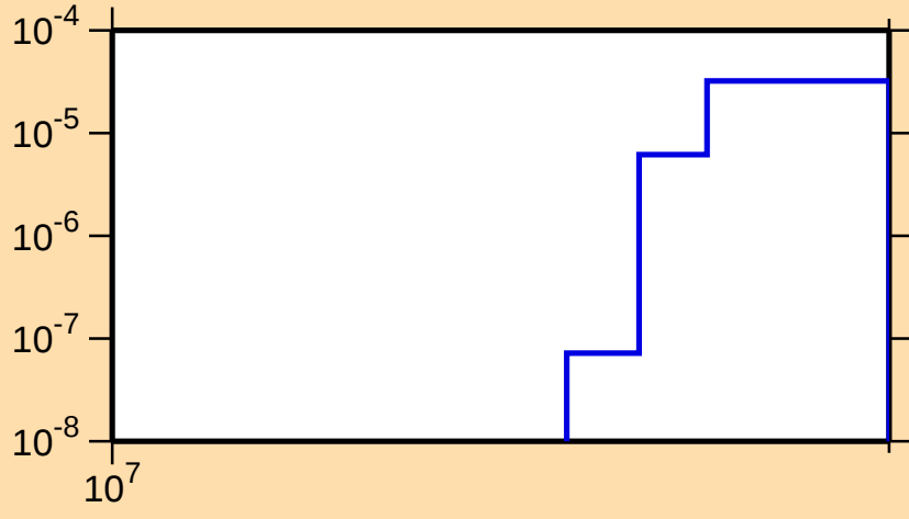
\sigma vs. E for ^{21}\text{O}(\text{n,t})
