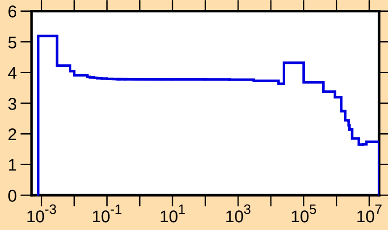
\sigma vs. E for ^{21}\text{O}(\text{n,tot.})
