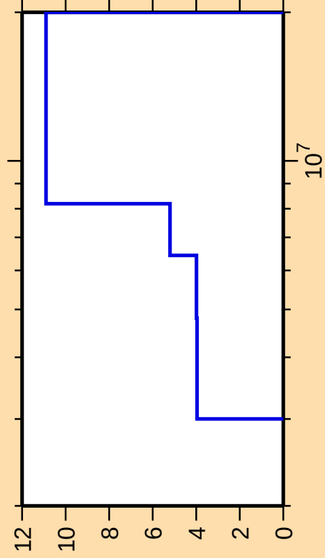
\Delta\sigma/\sigma vs. E for ^{21}\text{O}(n,n_1)
