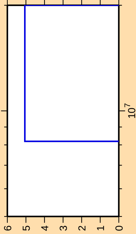
\Delta\sigma/\sigma vs. E for ^{21}\text{O}(\text{n,d})
