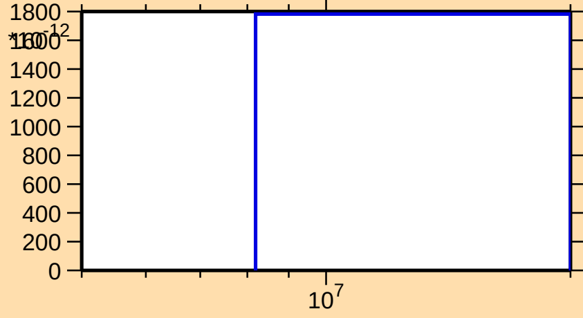
\sigma vs. E for ^{21}\text{O}(\text{n,p})
