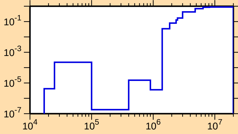
\sigma vs. E for ^{21}\text{O}(\text{n,nonel.})
