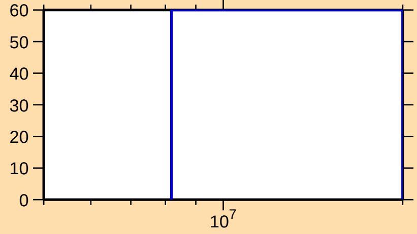
\Delta\sigma/\sigma vs. E for ^{21}\text{O}(n,p)
