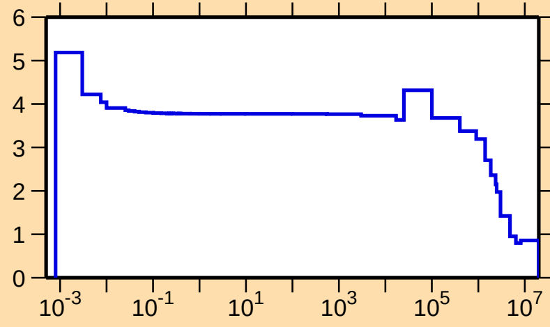
\sigma vs. E for ^{21}\text{O}(\text{n,el.})
