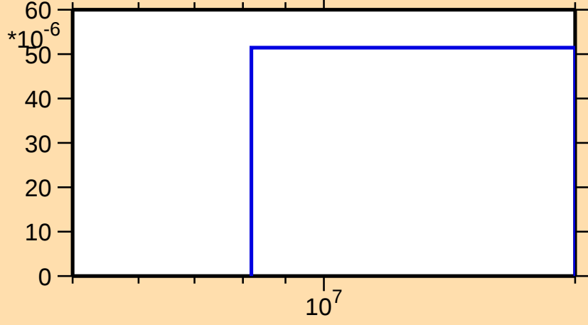
\sigma vs. E for ^{180}\text{Os}(n,3n)
