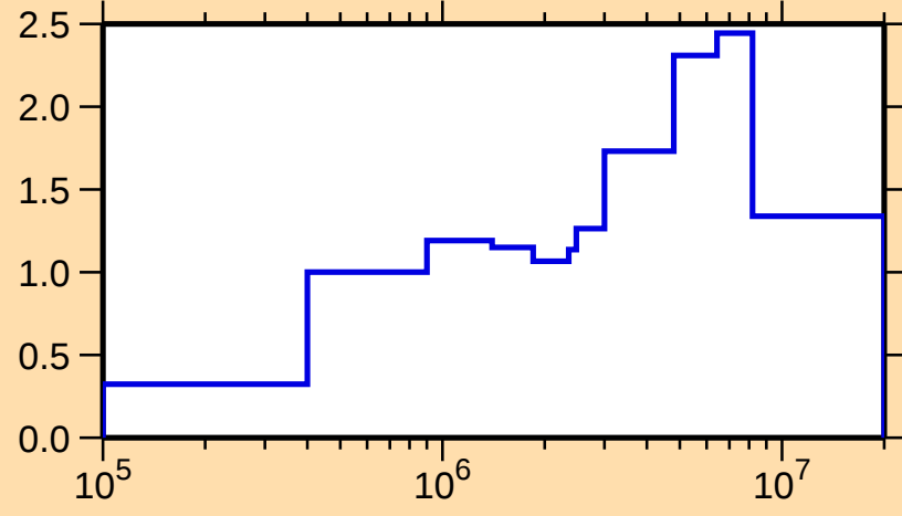
\sigma vs. E for ^{180}\text{Os}(n,\text{inel.})
