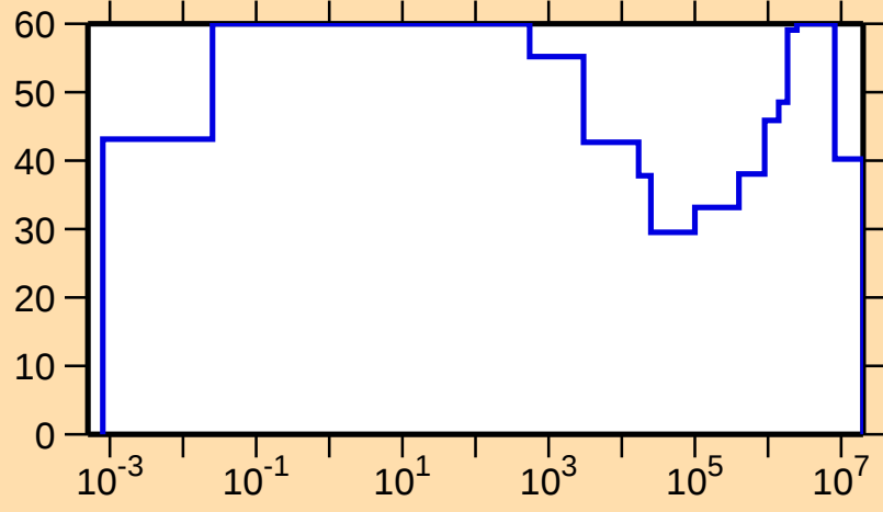
\Delta\sigma/\sigma vs. E for ^{180}\text{Os}(n,p)
