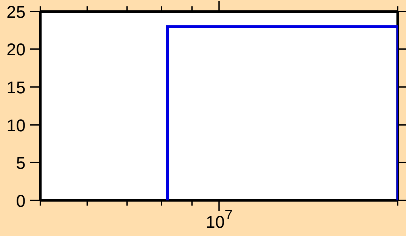
\Delta\sigma/\sigma vs. E for ^{180}\text{Os}(n,\text{inel.})
