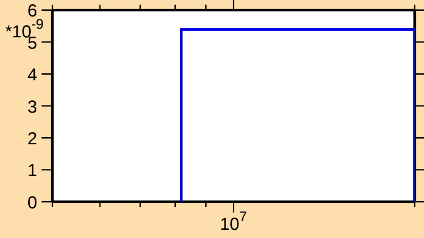
\sigma vs. E for ^{180}\text{Os}(n,\text{He}3)
