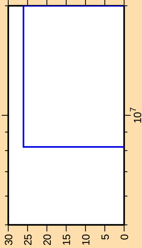
\Delta\sigma/\sigma vs. E for ^{180}\text{Os}(n,nt)
