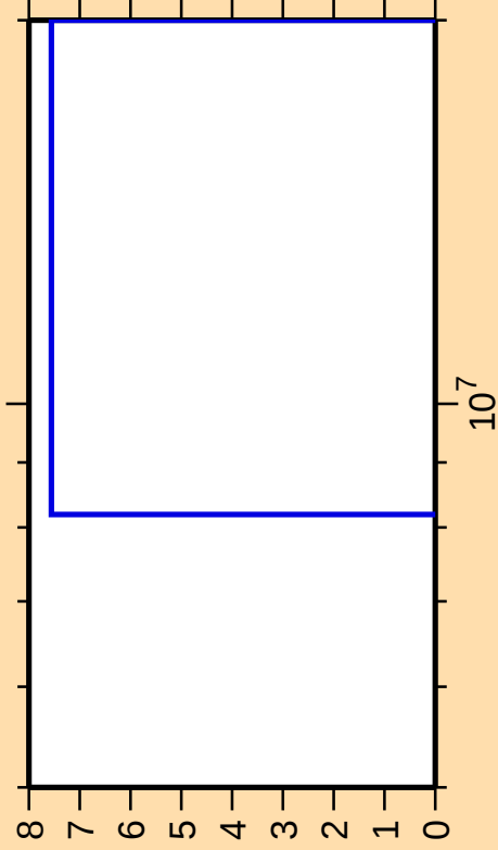
\Delta\sigma/\sigma vs. E for ^{180}\text{Os}(\text{mt117})
