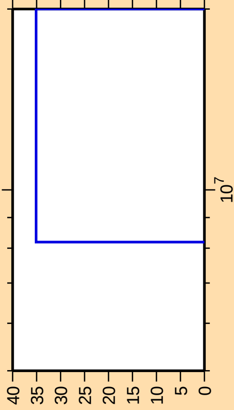
\Delta\sigma/\sigma vs. E for ^{180}\text{Os}(n,n_1)
