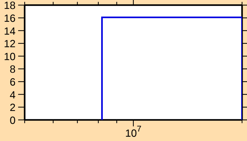
\Delta\sigma/\sigma vs. E for ^{180}\text{Os}(n,2n)
