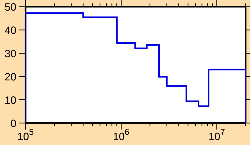
\Delta\sigma/\sigma vs. E for ^{180}\text{Os}(n,\text{inel.})
