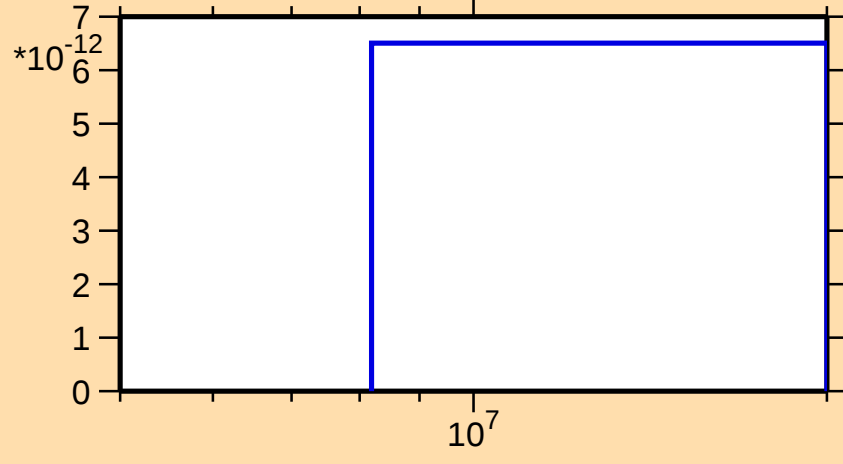
\sigma vs. E for ^{180}\text{Os}(n,\text{pd})
