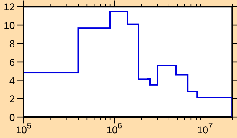
\Delta\sigma/\sigma vs. E for ^{180}\text{Os}(n,\text{tot.})
