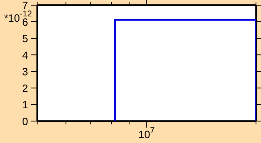
\sigma vs. E for ^{180}\text{Os}(n,nt)
