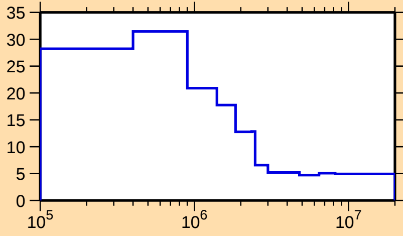
\Delta\sigma/\sigma vs. E for ^{180}\text{Os}(n,\text{nonel.})
