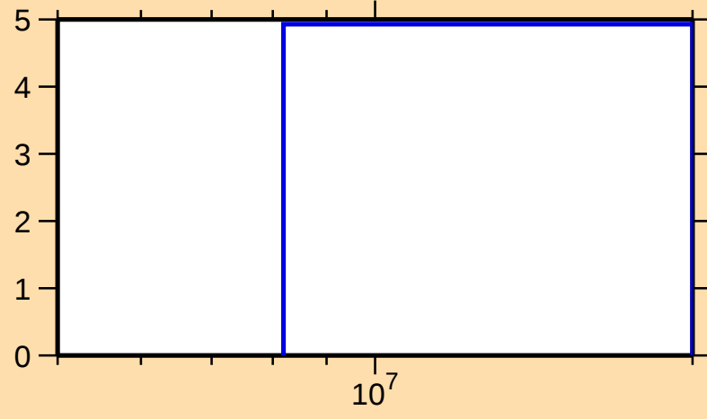
\Delta\sigma/\sigma vs. E for ^{180}\text{Os}(n,\text{nonel.})
