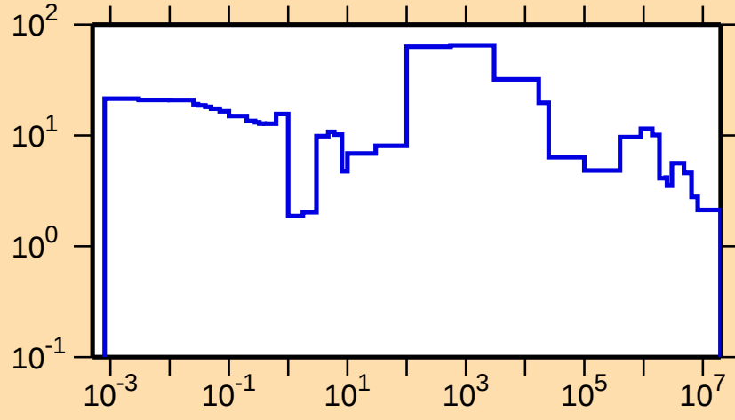
\Delta\sigma/\sigma vs. E for ^{180}\text{Os}(n,\text{tot.})
