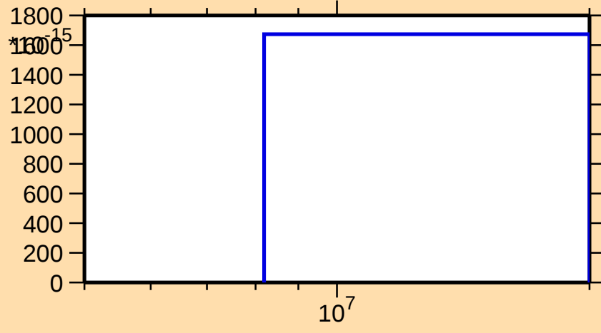
\sigma vs. E for ^{180}\text{Os}(\text{mt117})
