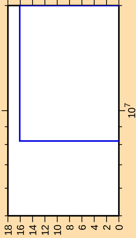
\Delta\sigma/\sigma vs. E for ^{180}\text{Os}(n,2n)
