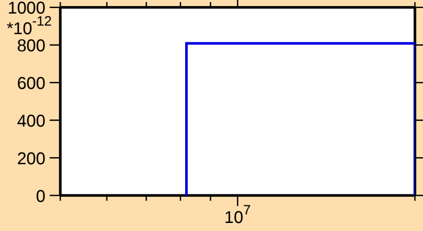
\sigma vs. E for ^{180}\text{Os}(n,\text{nd})
