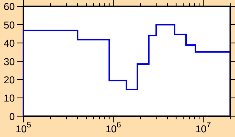
\Delta\sigma/\sigma vs. E for ^{180}\text{Os}(n,n_1)
