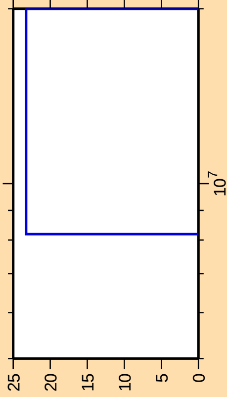
\Delta\sigma/\sigma vs. E for ^{180}\text{Os}(n,\text{pd})
