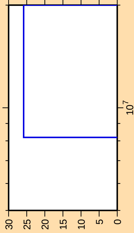
\Delta\sigma/\sigma vs. E for ^{180}\text{Os}(n,n\text{cont.})
