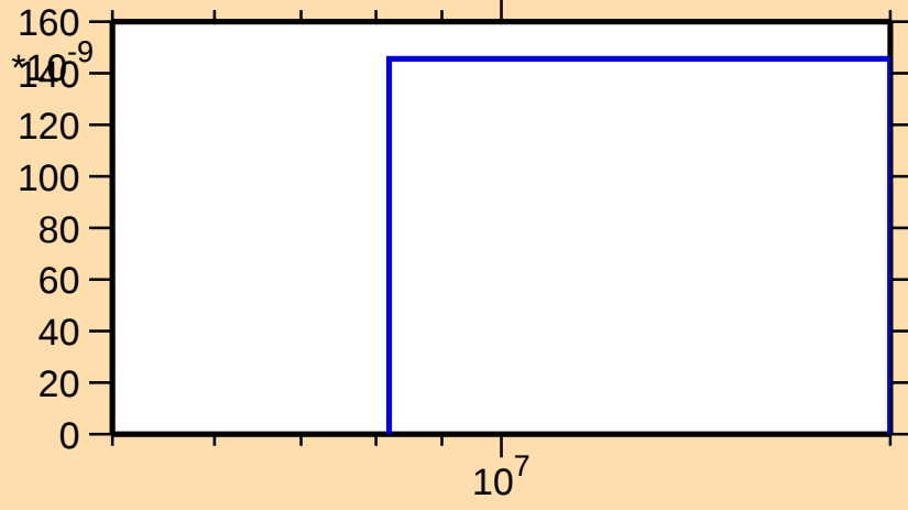
\sigma vs. E for ^{180}\text{Os}(n,2n\alpha)
