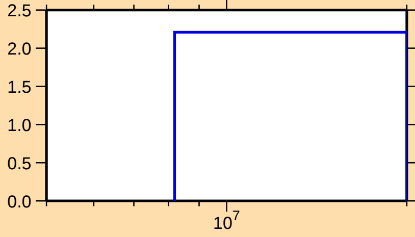
\Delta\sigma/\sigma vs. E for ^{180}\text{Os}(n,\text{el.})
