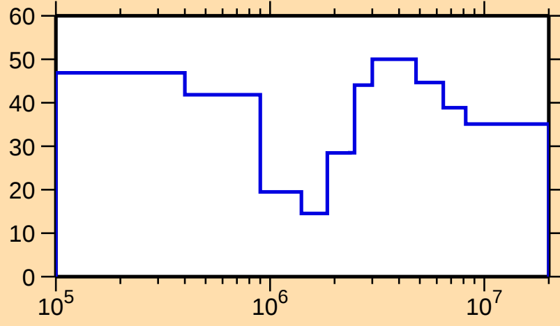
\Delta\sigma/\sigma vs. E for ^{180}\text{Os}(n,n_1)
