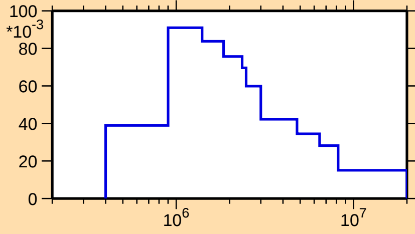
\sigma vs. E for ^{180}\text{Os}(n,n_2)
