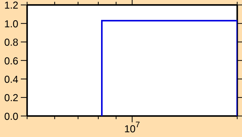
\sigma vs. E for ^{180}\text{Os}(n,2n)
