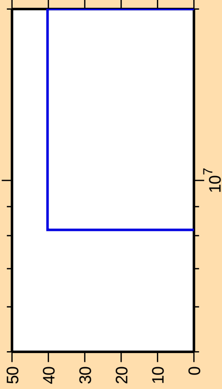
\Delta\sigma/\sigma vs. E for ^{180}\text{Os}(n,p)
