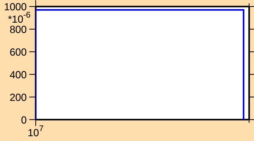
\sigma vs. E for ^{183}\text{Os}(n,3n)
