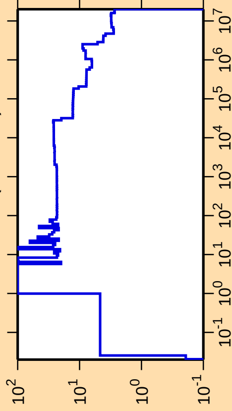
\Delta\sigma/\sigma vs. E for ^{189}\text{Os}(n,\text{nonel.})
