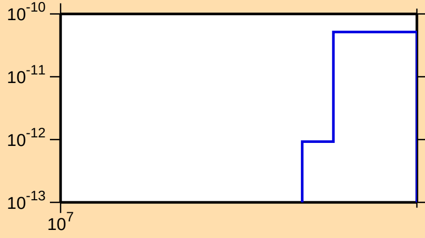
\sigma vs. E for ^{189}\text{Os}(n,\text{He}3)
