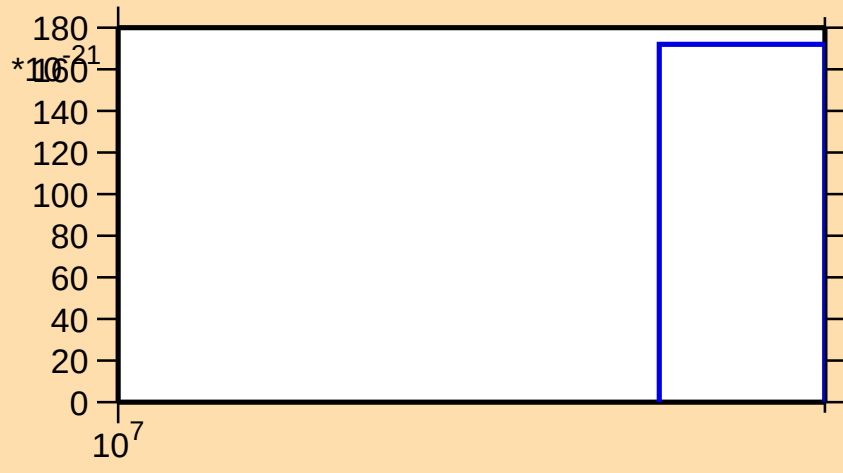
\sigma vs. E for ^{189}\text{Os}(\text{mt 11})
