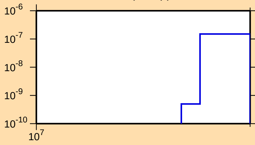
\sigma vs. E for ^{189}\text{Os}(n,2np)
