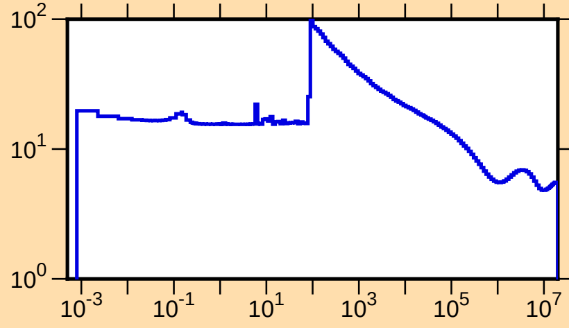
\sigma vs. E for ^{189}\text{Os}(n,\text{tot.})
