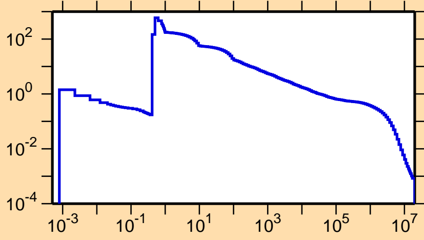
\sigma vs. E for ^{185}\text{Pb}(n,\gamma)
