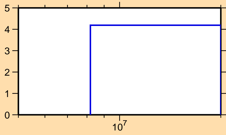
\Delta\sigma/\sigma vs. E for ^{185}\text{Pb}(n,\text{tot.})
