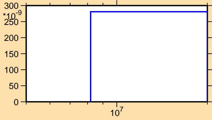
\sigma vs. E for ^{187}\text{Pb}(n,\text{pd})
