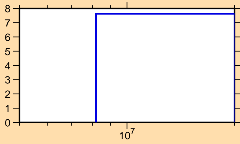
\Delta\sigma/\sigma vs. E for ^{187}\text{Pb}(n,\text{tot.})
