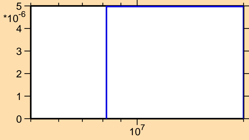
\sigma vs. E for ^{187}\text{Pb}(n,2n\alpha)
