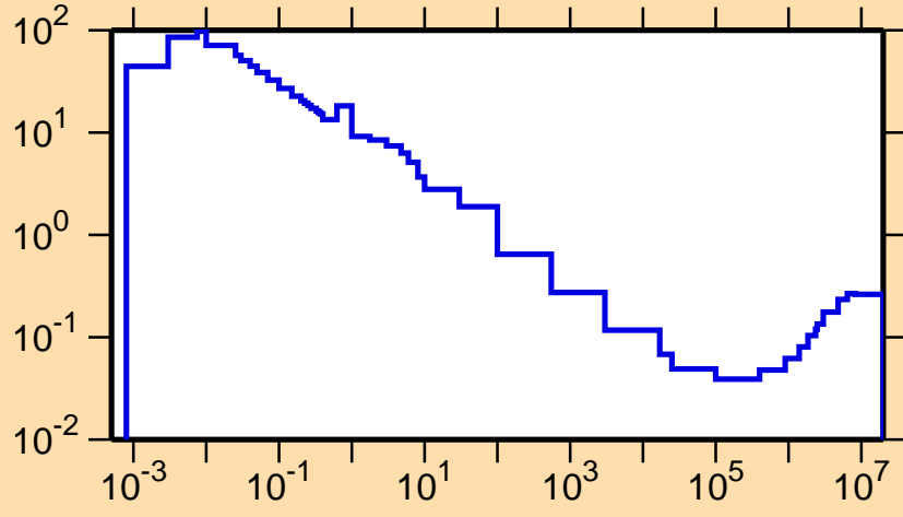
\sigma vs. E for ^{187}\text{Pb}(n,p)
