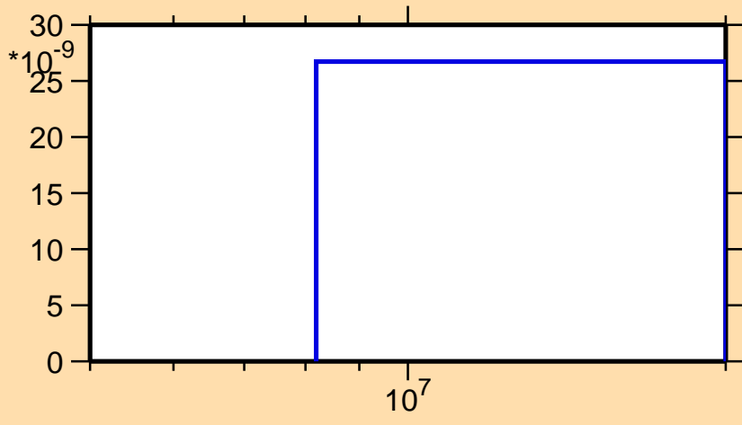
\sigma vs. E for ^{187}\text{Pb}(n,\text{nd})
