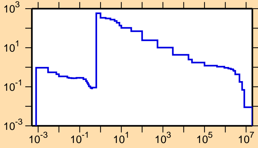
\sigma vs. E for ^{187}\text{Pb}(n,\gamma)
