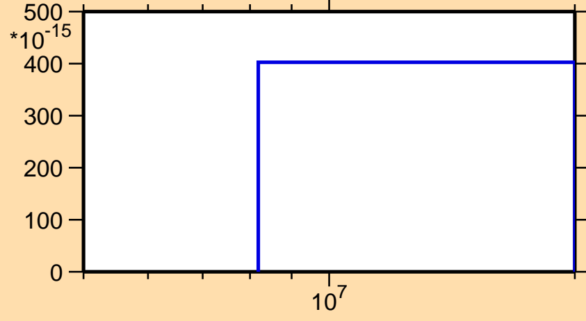
\sigma vs. E for ^{187}\text{Pb}(n,3n)
