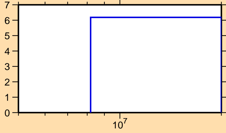
\Delta\sigma/\sigma vs. E for ^{187}\text{Pb}(n,\text{el.})
