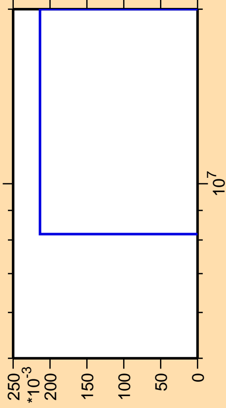
\Delta\sigma/\sigma vs. E for ^{187}\text{Pb}(n,nt)
