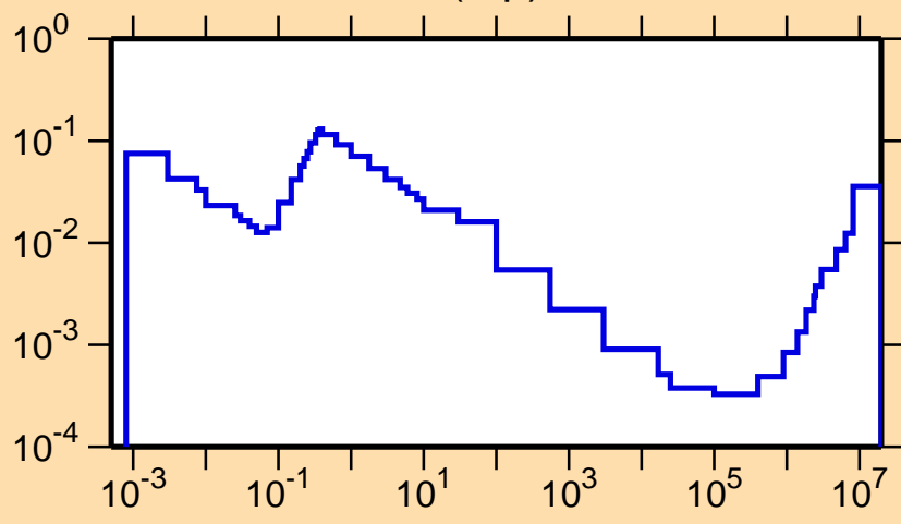
\sigma vs. E for ^{195}\text{Pb}(n,p)
