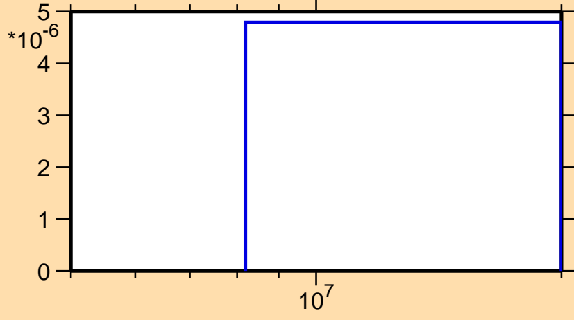
\sigma vs. E for ^{196}\text{Pb}(n,3n)
