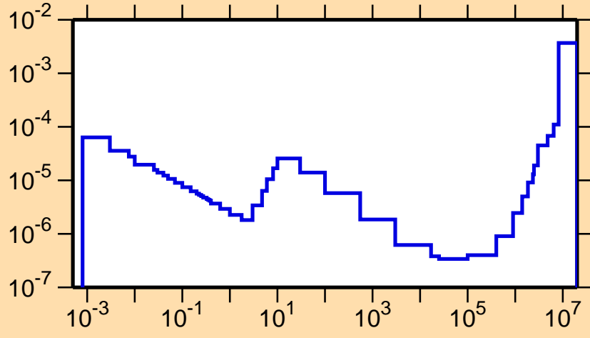
\sigma vs. E for ^{196}\text{Pb}(n,\alpha)
