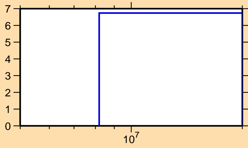
\Delta\sigma/\sigma vs. E for ^{196}\text{Pb}(n,\text{el.})
