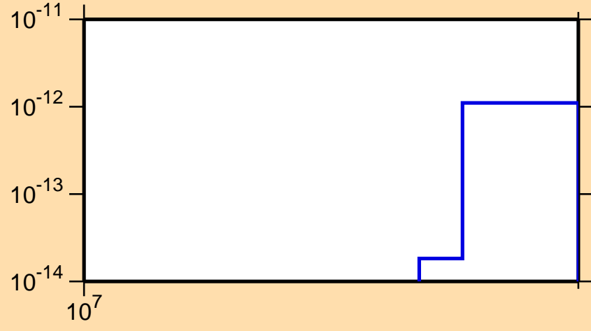
\sigma vs. E for ^{200}\text{Pb}(n,\text{pd})
