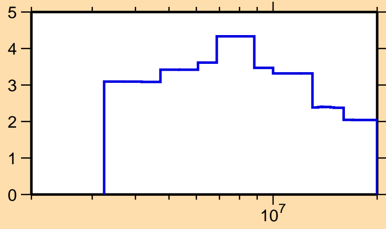
\Delta\sigma/\sigma vs. E for ^{200}\text{Pb}(n,\text{tot.})
