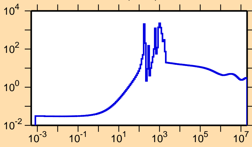
\sigma vs. E for ^{200}\text{Pb}(n,\text{el.})
