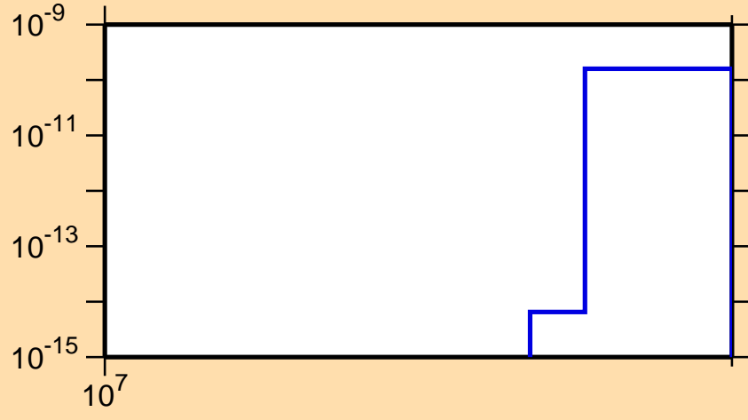
\sigma vs. E for ^{200}\text{Pb}(n,nt)
