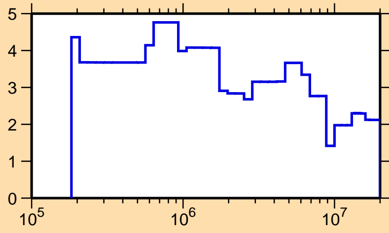
\Delta\sigma/\sigma vs. E for ^{200}\text{Pb}(n,\text{el.})
