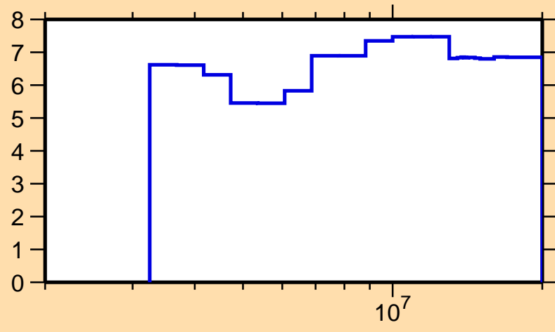
\Delta\sigma/\sigma vs. E for ^{200}\text{Pb}(n,\text{nonel.})
