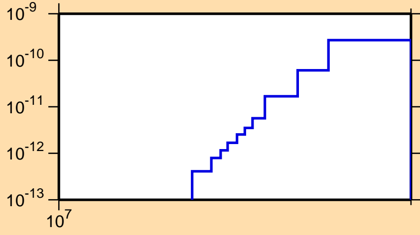
\sigma vs. E for ^{200}\text{Pb}(n,p\alpha)
