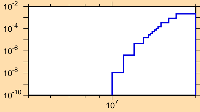
\sigma vs. E for ^{205}\text{Pb}(n,np)
