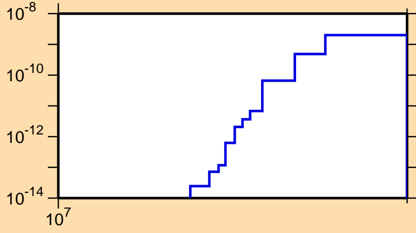
\sigma vs. E for ^{205}\text{Pb}(n,p\alpha)
