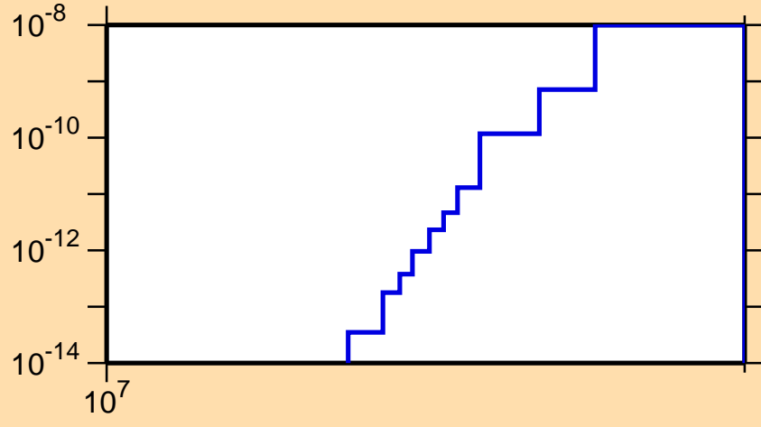
\sigma vs. E for ^{205}\text{Pb}(n,2n\alpha)
