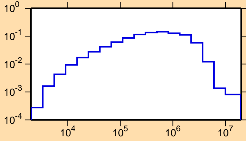
\sigma vs. E for ^{205}\text{Pb}(n,n_1)
