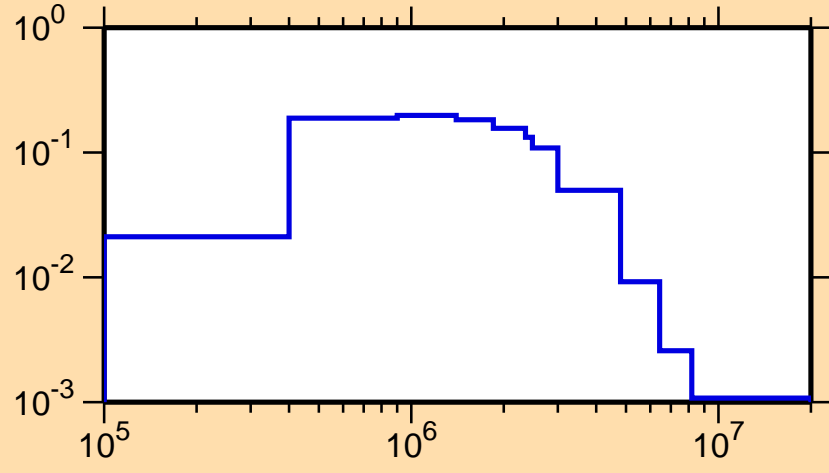
\sigma vs. E for ^{205}\text{Pb}(n,n_2)
