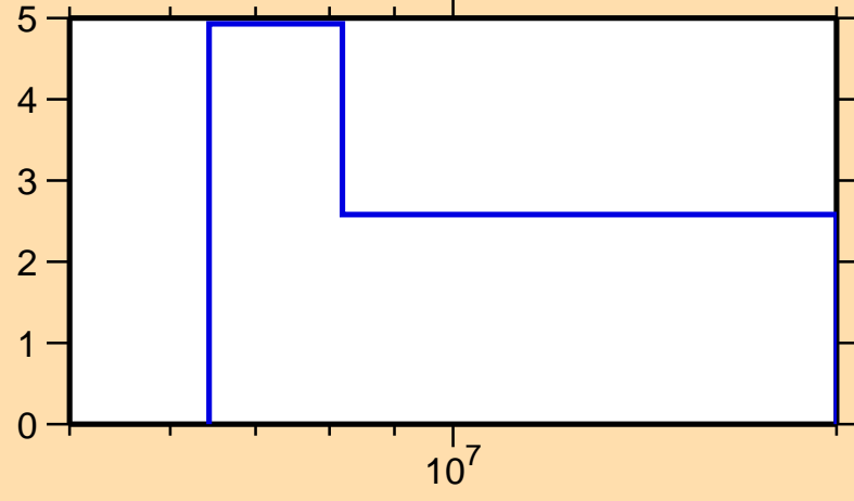
\Delta\sigma/\sigma vs. E for ^{205}\text{Pb}(n,\text{el.})
