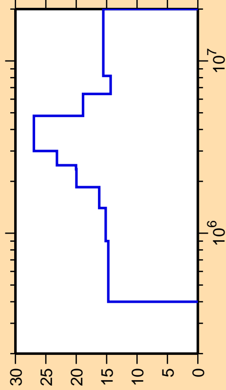
\Delta\sigma/\sigma vs. E for ^{205}\text{Pb}(n,n_4)
