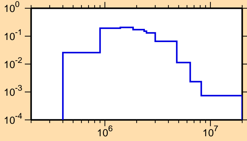
\sigma vs. E for ^{205}\text{Pb}(n,n_4)
