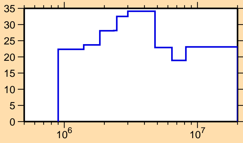
\Delta\sigma/\sigma vs. E for ^{205}\text{Pb}(n,\gamma)
