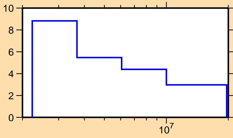
\Delta\sigma/\sigma vs. E for ^{215}\text{Pb}(n,\text{nonel.})
