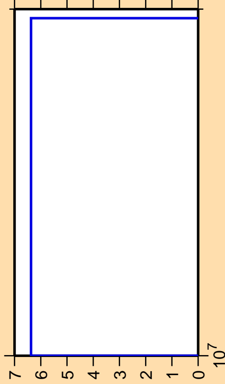
\Delta\sigma/\sigma vs. E for ^{215}\text{Pb}(n,3n\alpha)
