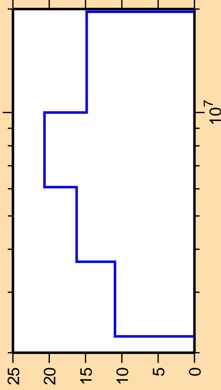
\Delta\sigma/\sigma vs. E for ^{215}\text{Pb}(n,n\text{cont.})
