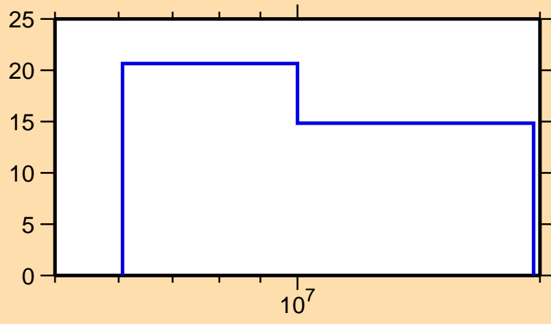
\Delta\sigma/\sigma vs. E for ^{215}\text{Pb}(n,n\text{cont.})
