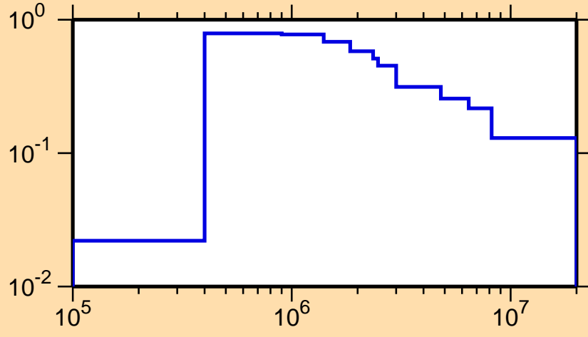
\sigma vs. E for ^{116}\text{Pd}(n,n_1)
