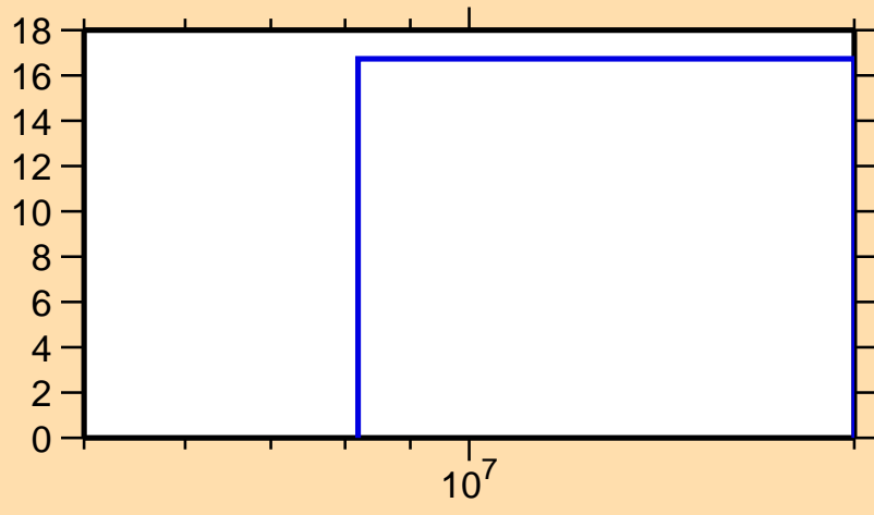
\Delta\sigma/\sigma vs. E for ^{116}\text{Pd}(n,n\text{cont.})
