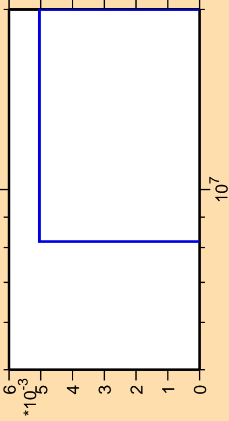
\Delta\sigma/\sigma vs. E for ^{116}\text{Pd}(n,2n\alpha)
