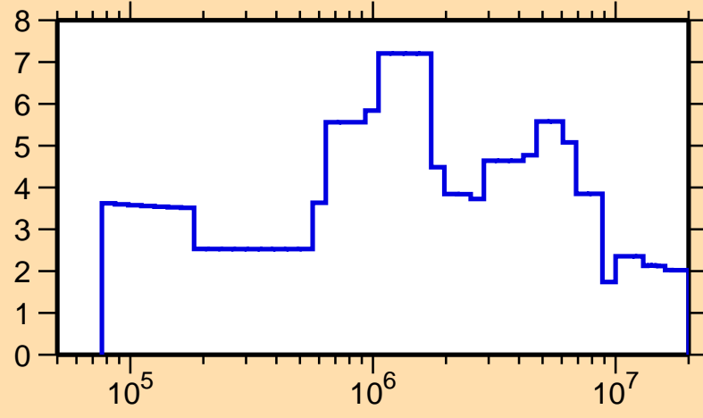
\Delta\sigma/\sigma vs. E for ^{211}\text{Po}(n, el.)
