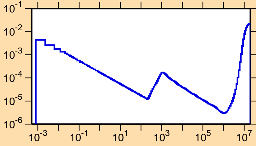
\sigma vs. E for ^{211}\text{Po}(n,\alpha)
