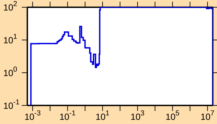
\Delta\sigma/\sigma vs. E for ^{127}\text{Pr}(n,\gamma)
