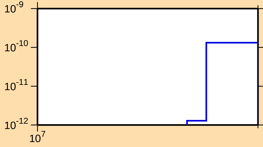
\sigma vs. E for ^{127}\text{Pr}(\text{mt 34})
