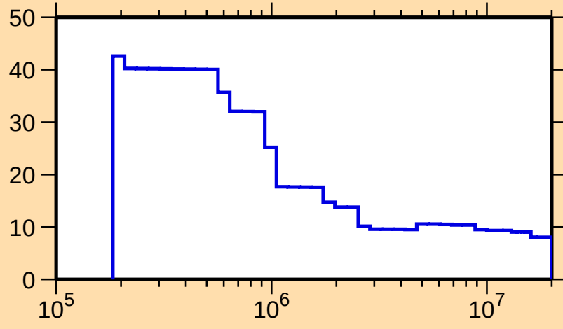
\Delta\sigma/\sigma vs. E for ^{127}\text{Pr}(\text{n},\text{nonel.})
