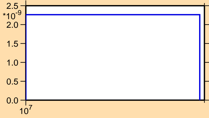
\sigma vs. E for ^{127}\text{Pr}(n,\text{pt})
