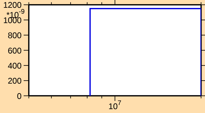
\sigma vs. E for ^{127}\text{Pr}(n,2np)
