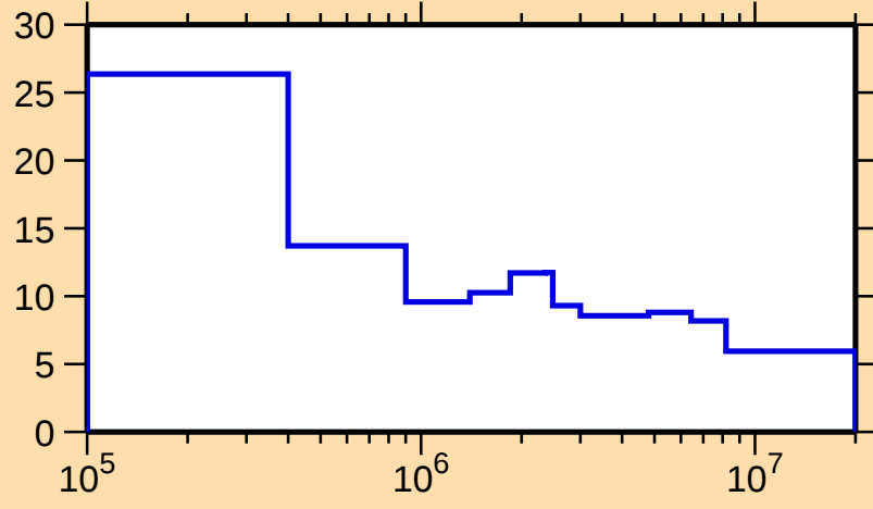
\Delta\sigma/\sigma vs. E for ^{127}\text{Pr}(n,\text{tot.})
