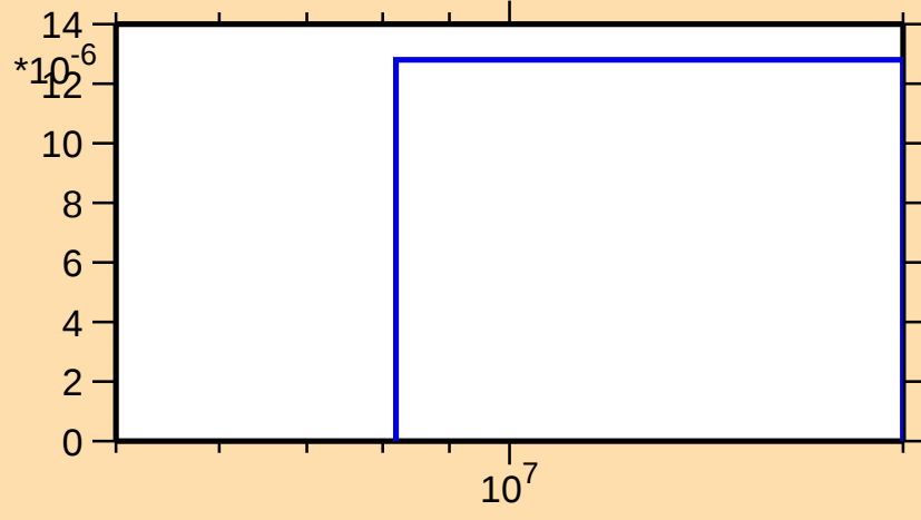
\sigma vs. E for ^{127}\text{Pr}(\text{mt } 45)
