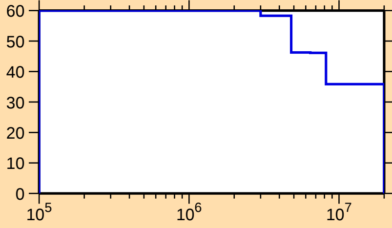
\Delta\sigma/\sigma vs. E for ^{127}\text{Pr}(n,n_1)
