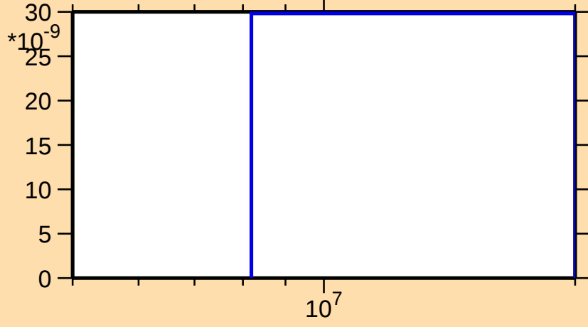
\sigma vs. E for ^{127}\text{Pr}(n,\text{nd})
