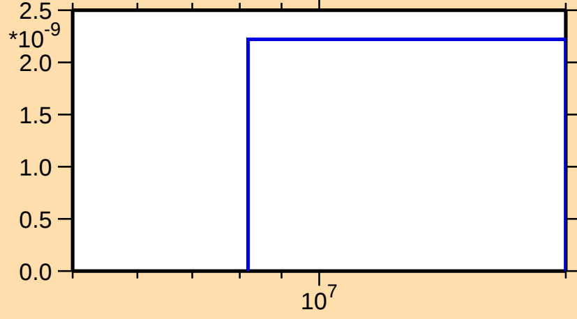
\sigma vs. E for ^{127}\text{Pr}(n,\text{pt})
