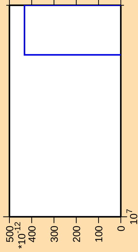
\Delta\sigma/\sigma vs. E for ^{131}\text{Pr}(\text{mt } 11)
