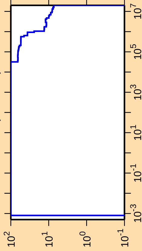
\Delta\sigma/\sigma vs. E for ^{131}\text{Pr}(n,\text{nonel.})
