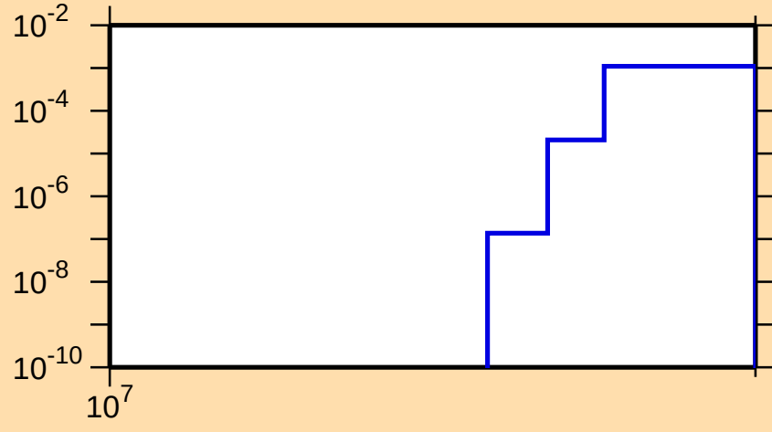
\sigma vs. E for ^{131}\text{Pr}(n,2np)
