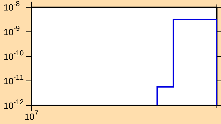
\sigma vs. E for ^{131}\text{Pr}(n,\text{pt})
