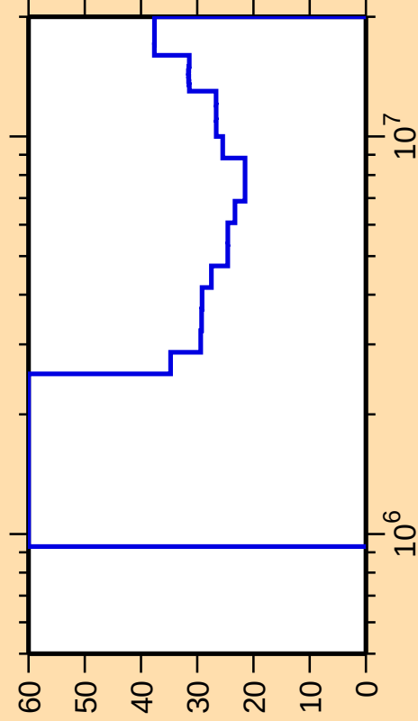
\Delta\sigma/\sigma vs. E for ^{131}\text{Pr}(n,\text{ncont.})
