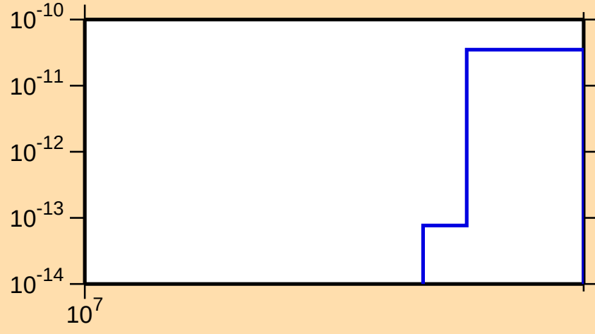
\sigma vs. E for ^{131}\text{Pr}(\text{mt 34})
