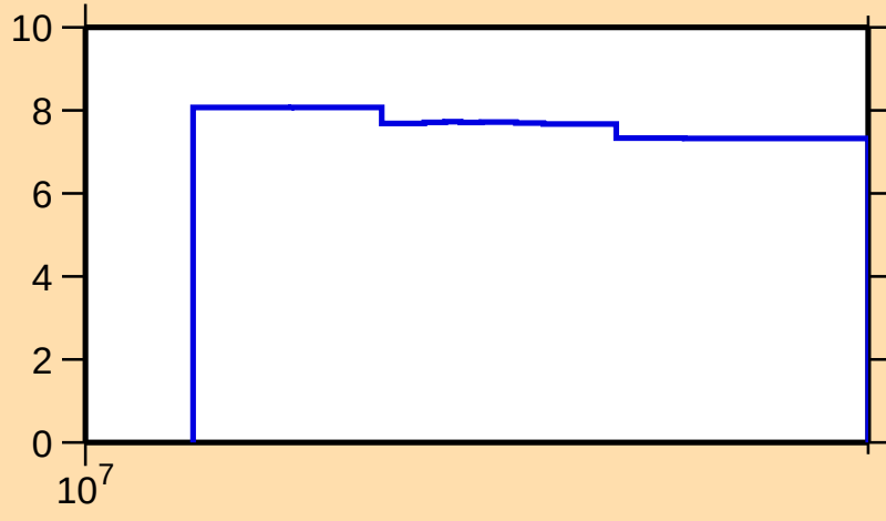
\Delta\sigma/\sigma vs. E for ^{131}\text{Pr}(n,\text{nonel.})
