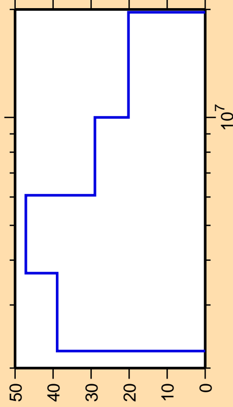
\Delta\sigma/\sigma vs. E for ^{131}\text{Pr}(n,np)
