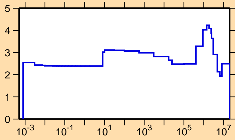
\sigma vs. E for ^{131}\text{Pr}(n,\text{el.})
