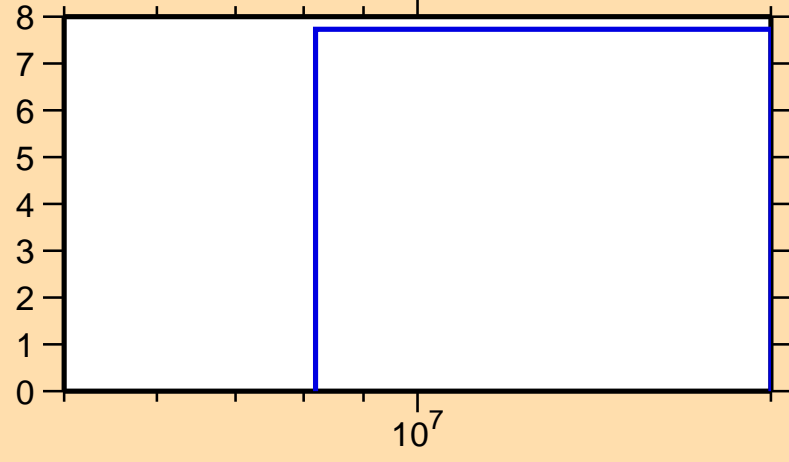
\Delta\sigma/\sigma vs. E for ^{131}\text{Pr}(n,\text{el.})
