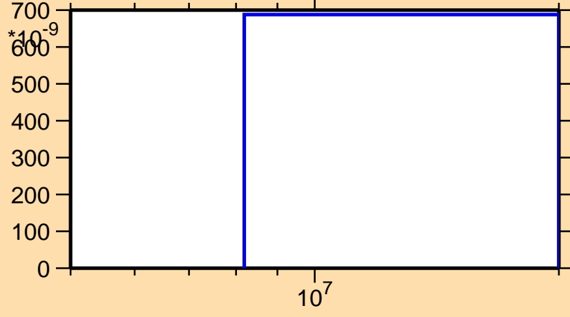
\sigma vs. E for ^{131}\text{Pr}(n,pd)
