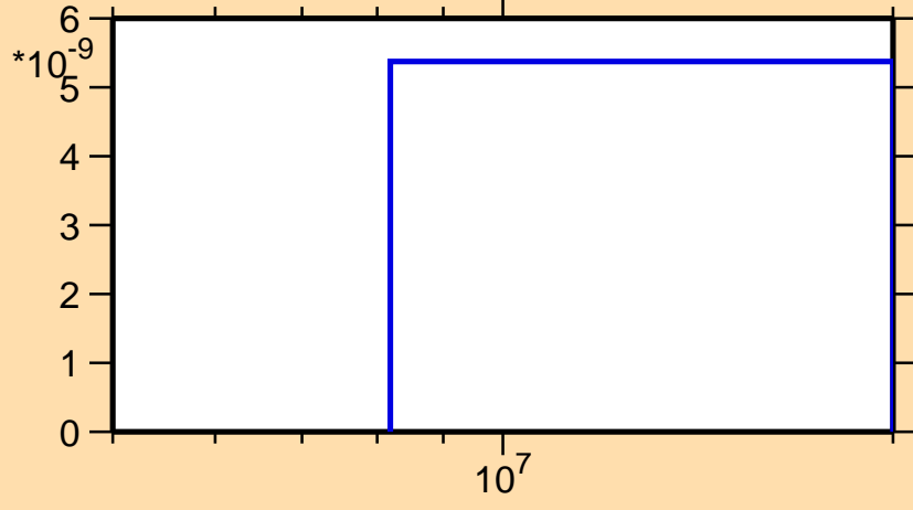
\sigma vs. E for ^{131}\text{Pr}(\text{mt117})
