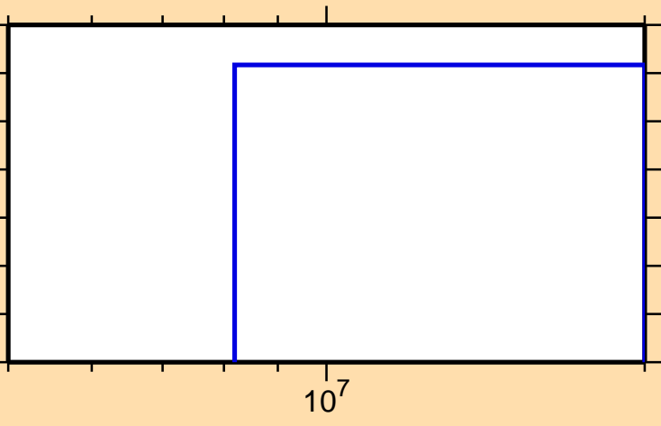
\sigma vs. E for ^{134}\text{Pr}(n,3n)
