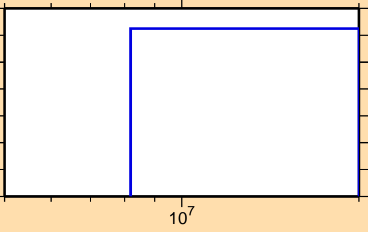
\sigma vs. E for ^{134}\text{Pr}(n,2n\alpha)
