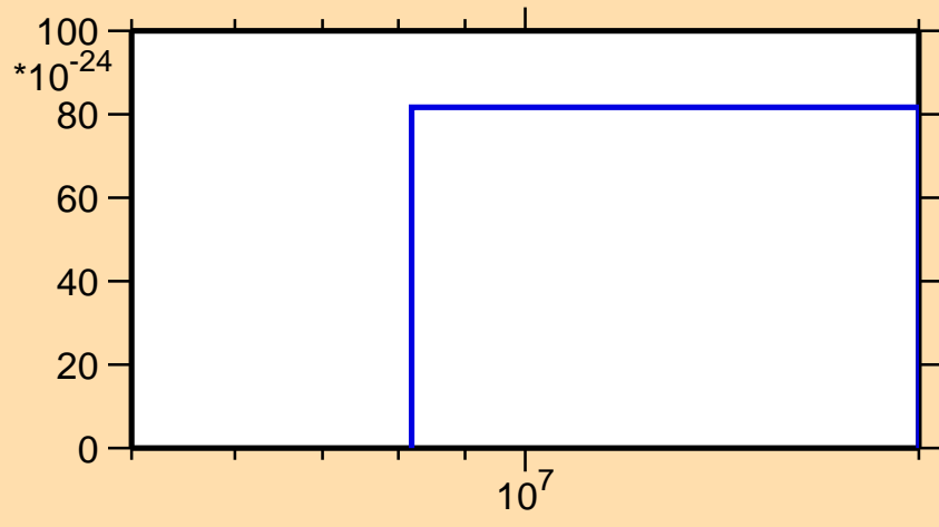
\sigma vs. E for ^{134}\text{Pr}(\text{mt 11})
