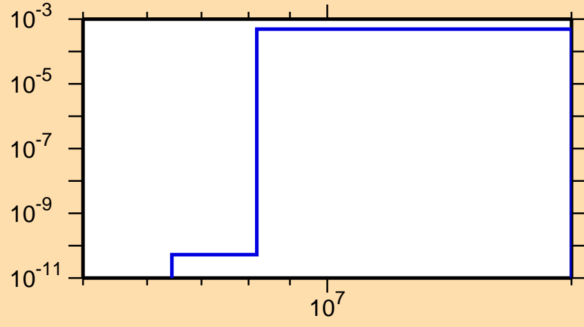
\sigma vs. E for ^{134}\text{Pr}(n,t)
