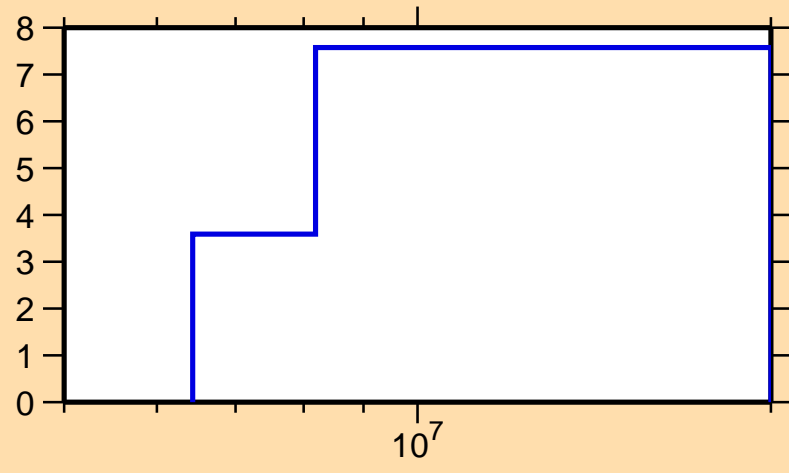
\Delta\sigma/\sigma vs. E for ^{140}\text{Pr}(n,\text{inel.})
