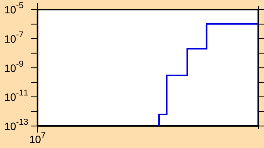
\sigma vs. E for ^{141}\text{Pr}(n,\text{nd})
