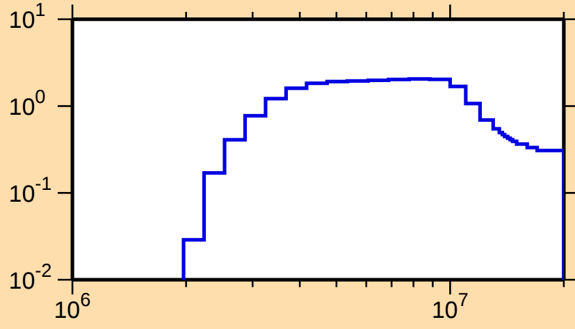
\sigma vs. E for ^{141}\text{Pr}(n,n\text{cont.})
