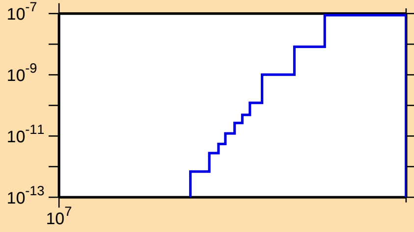
\sigma vs. E for ^{141}\text{Pr}(n,\text{He3})
