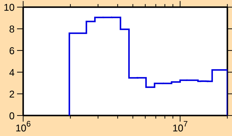
\Delta\sigma/\sigma vs. E for ^{141}\text{Pr}(n,\text{el.})
