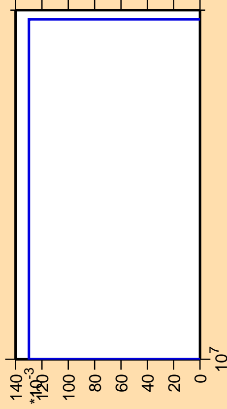
\Delta\sigma/\sigma vs. E for ^{149}\text{Pr}(n,3n\alpha)
