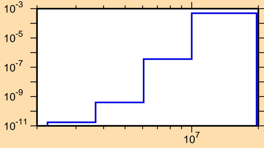
\sigma vs. E for ^{149}\text{Pr}(n,\alpha)
