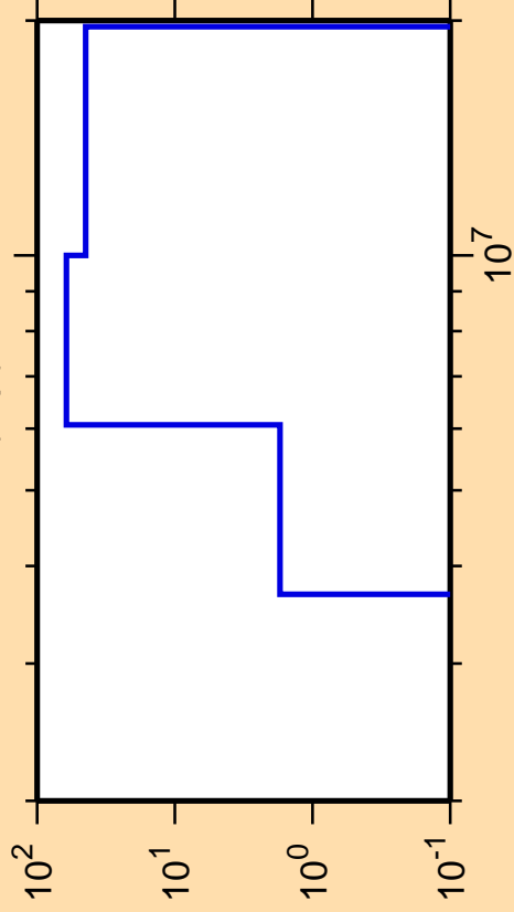
\Delta\sigma/\sigma vs. E for ^{149}\text{Pr}(n,p)
