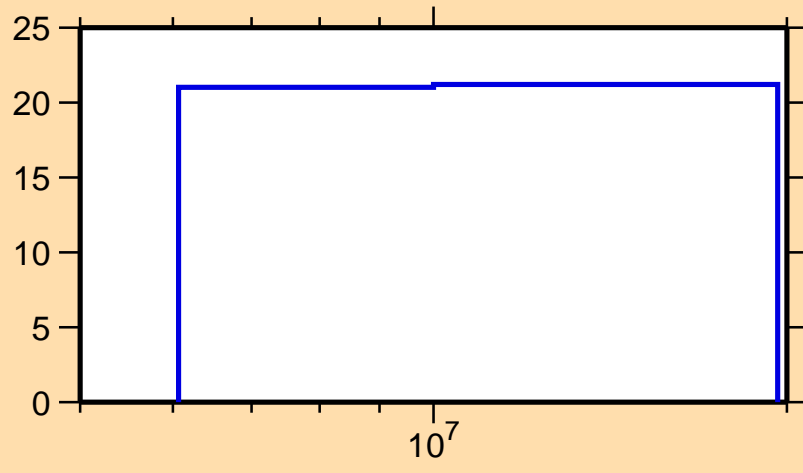
\Delta\sigma/\sigma vs. E for ^{149}\text{Pr}(n,\text{inel.})
