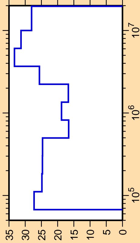
\Delta\sigma/\sigma vs. E for ^{149}\text{Pr}(n,n_4)
