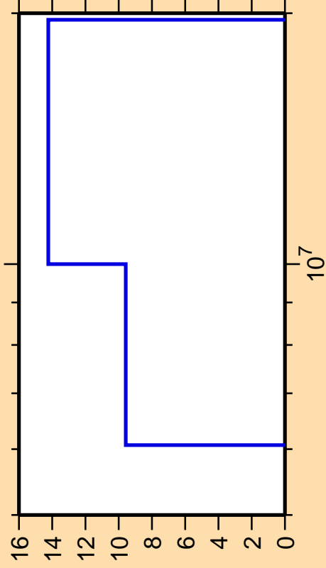
\Delta\sigma/\sigma vs. E for ^{149}\text{Pr}(n,2n)
