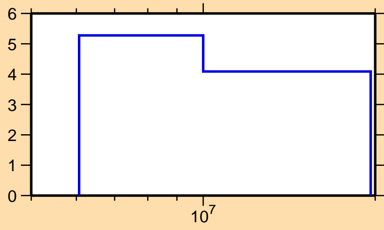
\Delta\sigma/\sigma vs. E for ^{149}\text{Pr}(n,\text{tot.})
