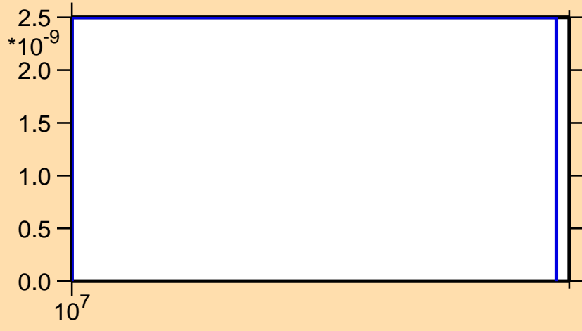
\sigma vs. E for ^{149}\text{Pr}(n,2n\alpha)
