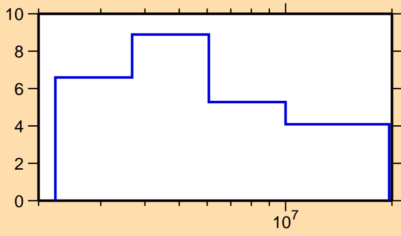
\Delta\sigma/\sigma vs. E for ^{149}\text{Pr}(n,\text{tot.})
