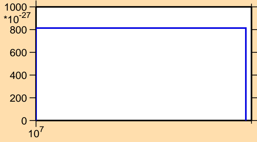
\sigma vs. E for ^{149}\text{Pr}(\text{mt } 42)
