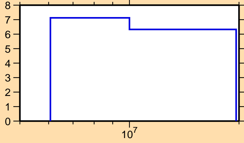
\Delta\sigma/\sigma vs. E for ^{149}\text{Pr}(n,\text{el.})
