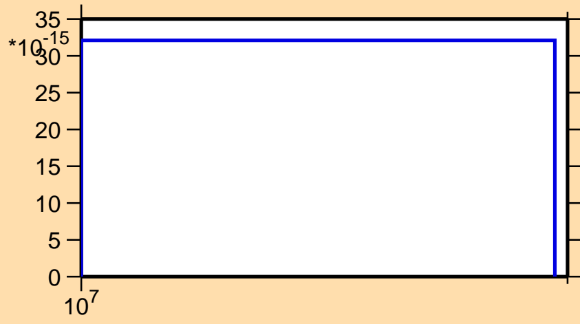
\sigma vs. E for ^{149}\text{Pr}(n,3n\alpha)
