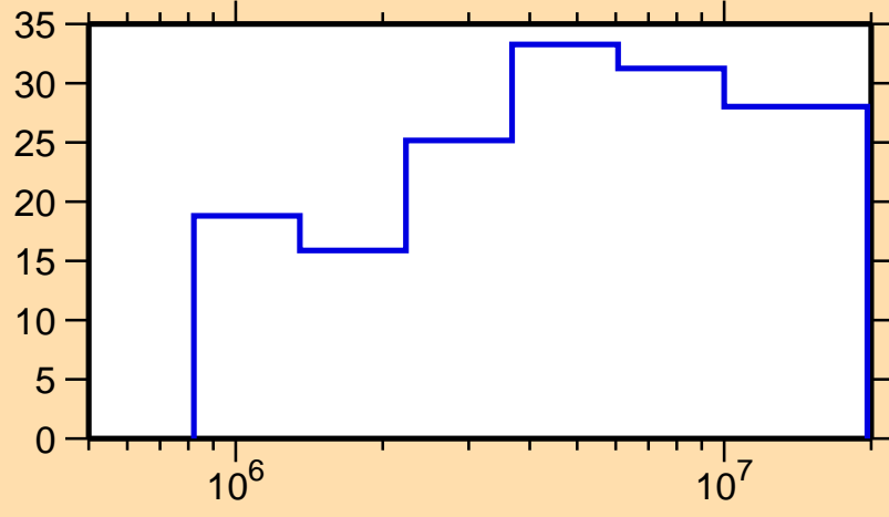
\Delta\sigma/\sigma vs. E for ^{149}\text{Pr}(n,n_1)
