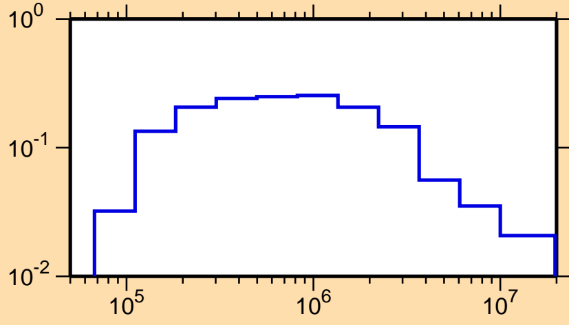
\sigma vs. E for ^{149}\text{Pr}(n,n_4)
