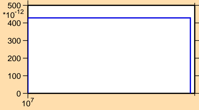
\sigma vs. E for ^{149}\text{Pr}(n,2np)
