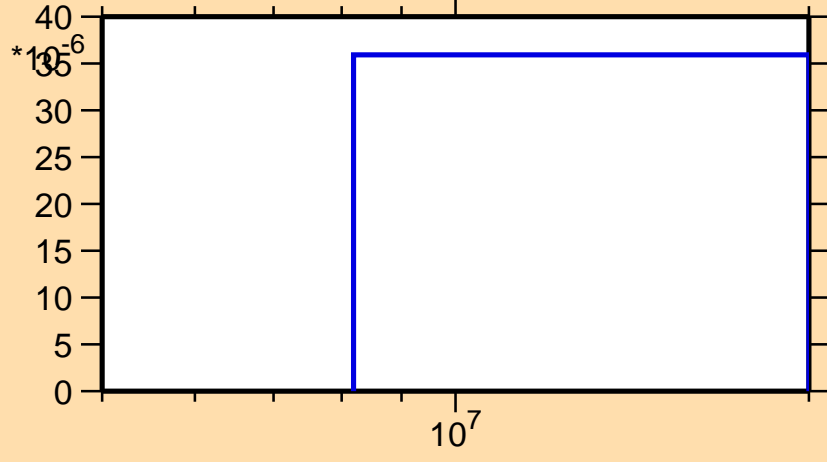
\sigma vs. E for ^{149}\text{Pr}(n,t)
