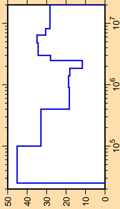
\Delta\sigma/\sigma vs. E for ^{149}\text{Pr}(n,n_1)
