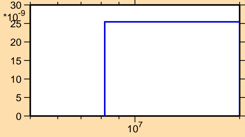
\sigma vs. E for ^{149}\text{Pr}(n,\text{nd})
