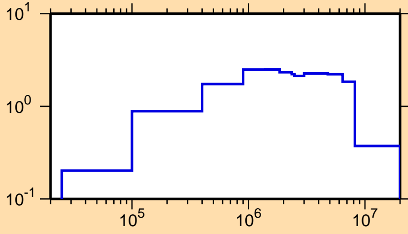
\sigma vs. E for ^{149}\text{Pr}(n,\text{inel.})
