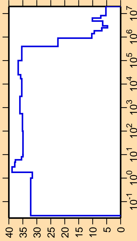
\Delta\sigma/\sigma vs. E for ^{149}\text{Pr}(n,\text{nonel.})
