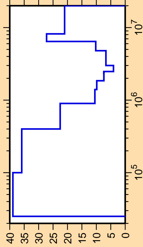
\Delta\sigma/\sigma vs. E for ^{149}\text{Pr}(n,\text{inel.})
