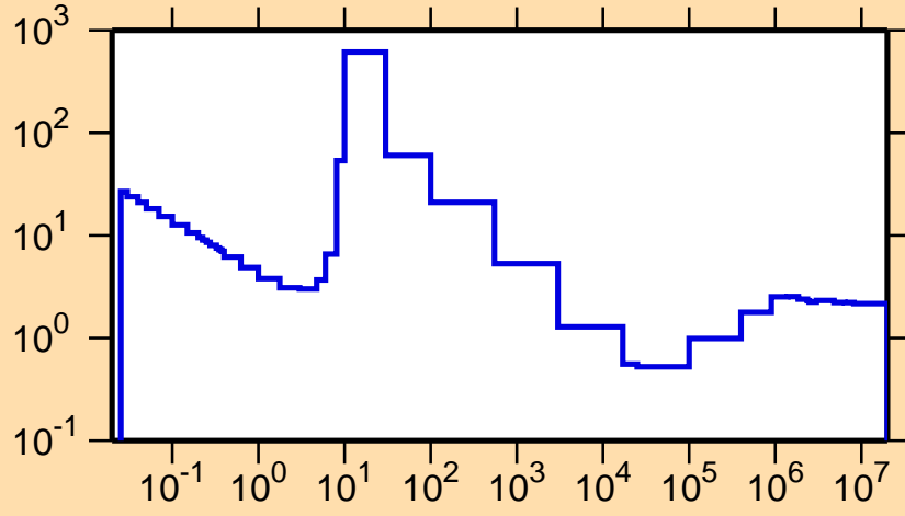
\sigma vs. E for ^{149}\text{Pr}(n,\text{nonel.})
