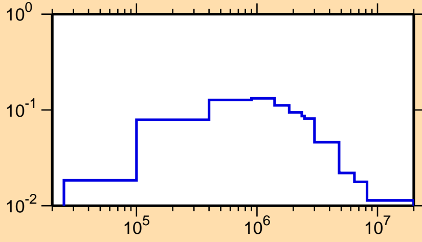
\sigma vs. E for ^{149}\text{Pr}(n,n_1)
