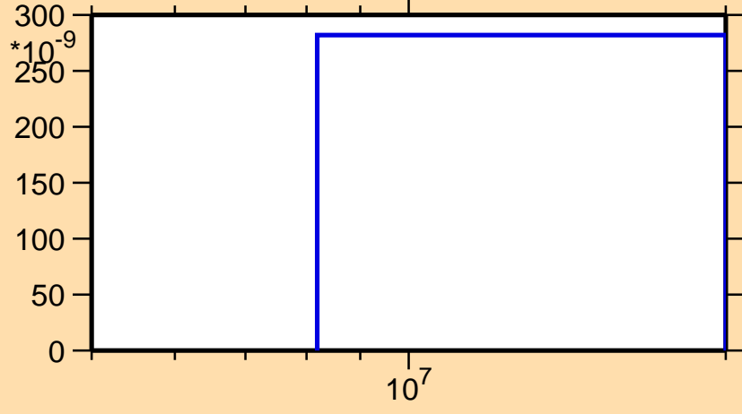
\sigma vs. E for ^{149}\text{Pr}(n,nt)
