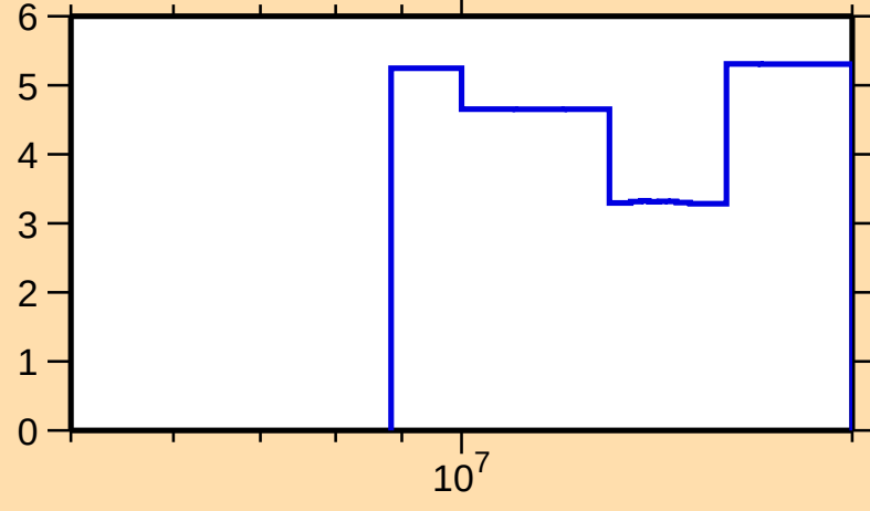
\Delta\sigma/\sigma vs. E for ^{204}\text{Pt}(n,\text{tot.})
