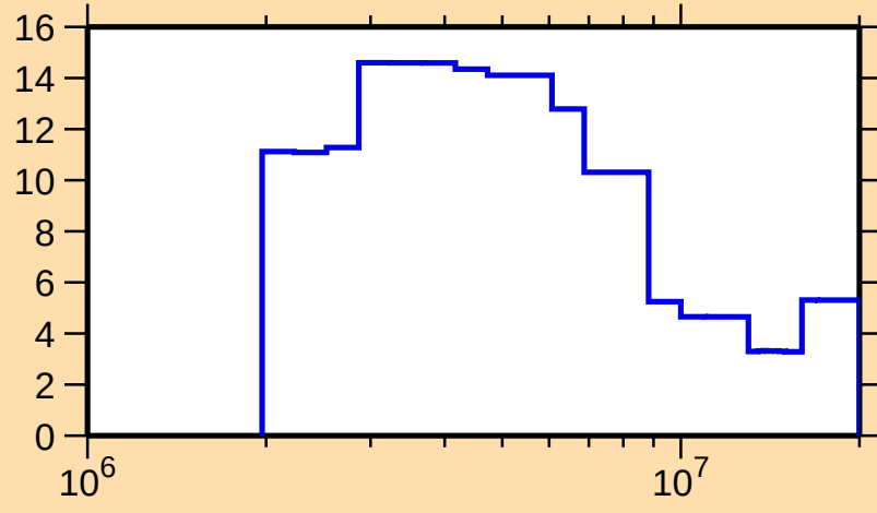
\Delta\sigma/\sigma vs. E for ^{204}\text{Pt}(n,\text{tot.})
