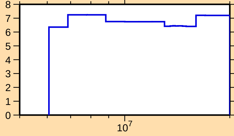
\Delta\sigma/\sigma vs. E for ^{204}\text{Pt}(n,\text{nonel.})
