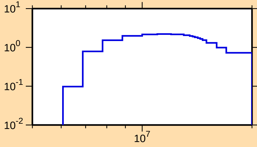
\sigma vs. E for ^{204}\text{Pt}(n,2n)
