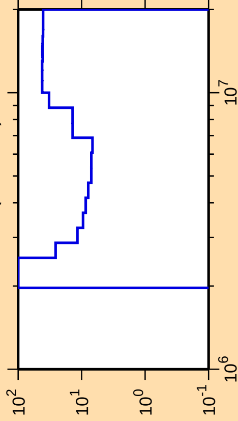
\Delta\sigma/\sigma vs. E for ^{204}\text{Pt}(n,\text{ncont.})
