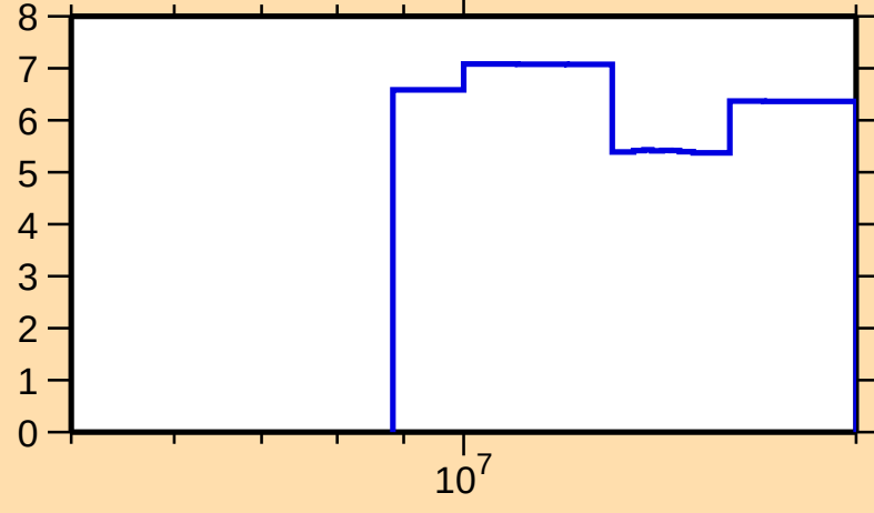
\Delta\sigma/\sigma vs. E for ^{204}\text{Pt}(n,\text{el.})
