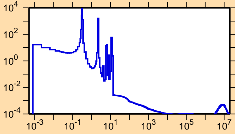
\sigma vs. E for ^{232}\text{Pu}(n,\gamma)
