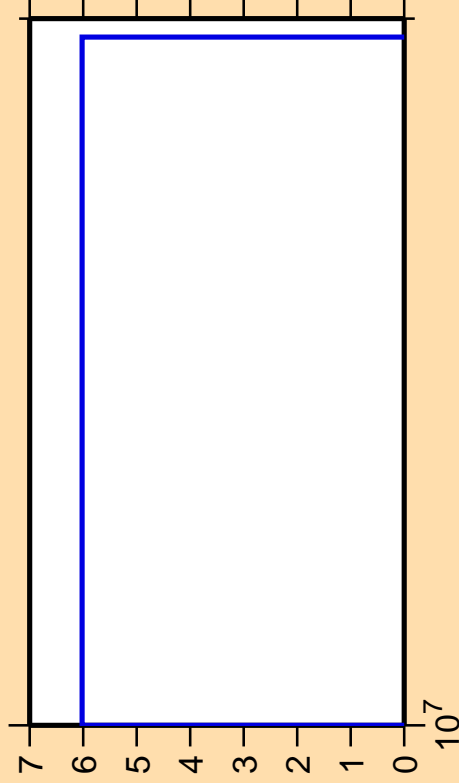
\Delta\sigma/\sigma vs. E for ^{232}\text{Pu}(n,2np)
