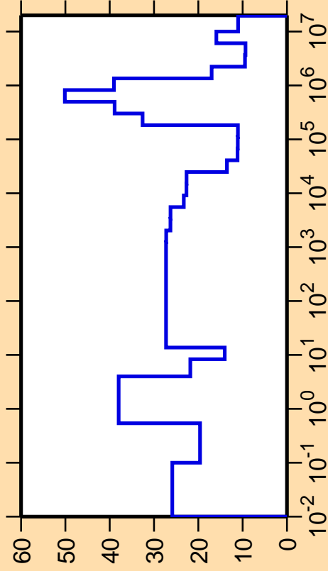
\Delta\sigma/\sigma vs. E for ^{232}\text{Pu}(n,\text{el.})
