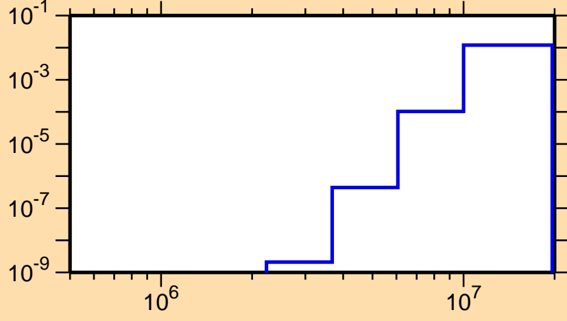
\sigma vs. E for ^{232}\text{Pu}(n,p)
