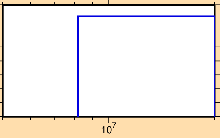
\sigma vs. E for ^{232}\text{Pu} (mt 42)
