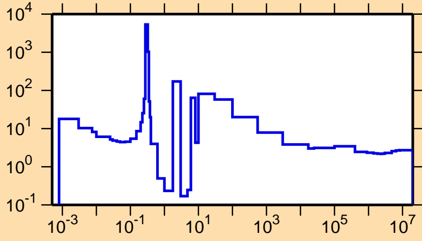
\sigma vs. E for ^{232}\text{Pu}(n,f)
