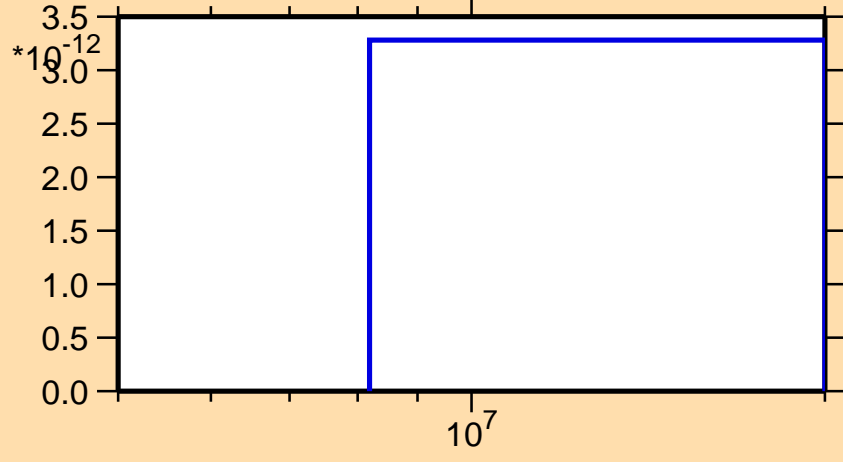
\sigma vs. E for ^{232}\text{Pu}(n,nd)
