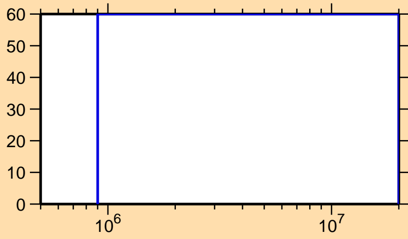
\Delta\sigma/\sigma vs. E for ^{232}\text{Pu}(n,\gamma)
