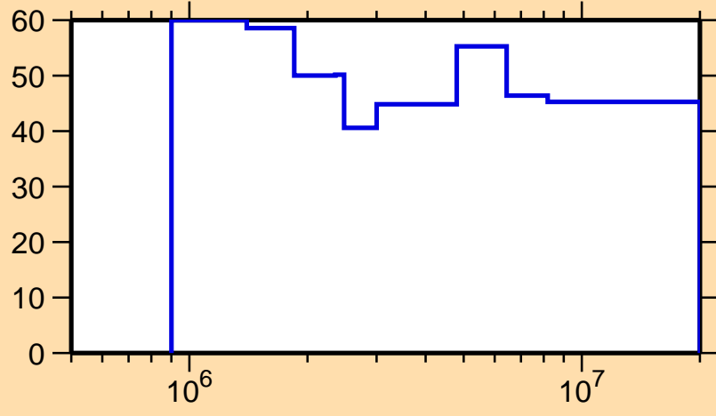
\Delta\sigma/\sigma vs. E for ^{232}\text{Pu}(n,n_1)
