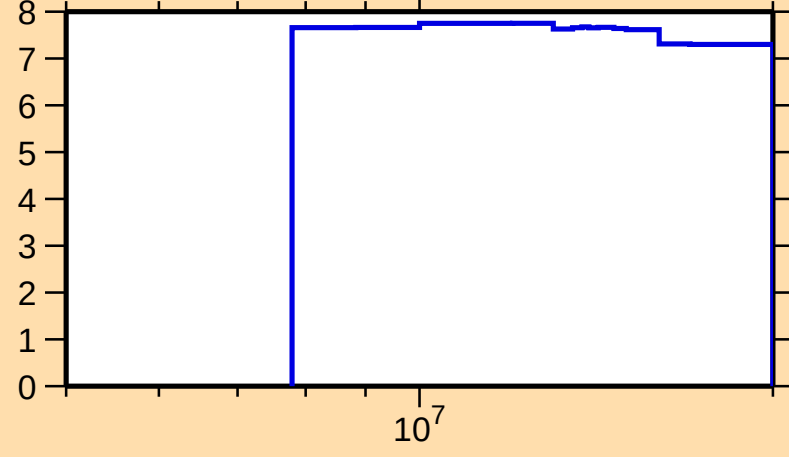
\Delta\sigma/\sigma vs. E for ^{234}\text{Pu}(n,\text{nonel.})
