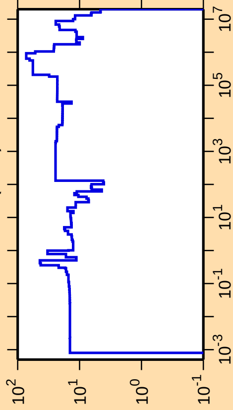
\Delta\sigma/\sigma vs. E for ^{234}\text{Pu}(n,\text{el.})
