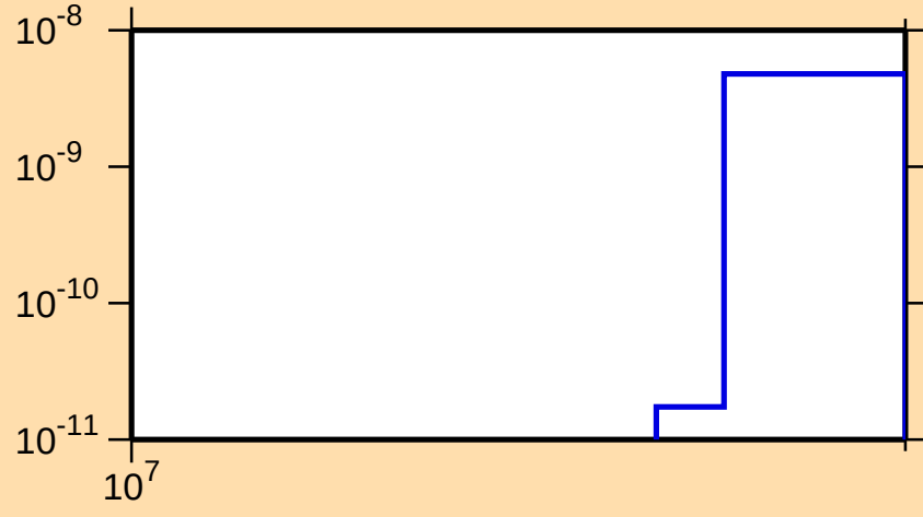
\sigma vs. E for ^{234}\text{Pu}(n,2np)
