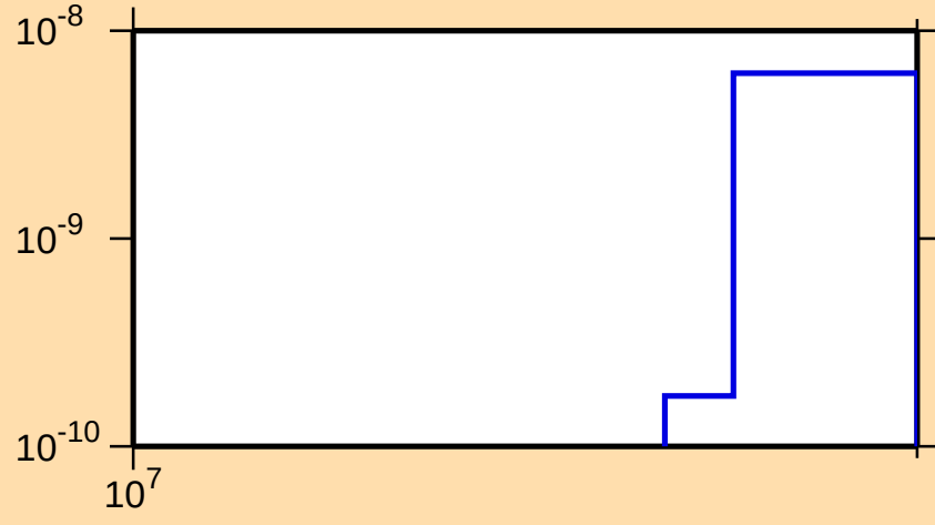
\sigma vs. E for ^{234}\text{Pu}(n,\text{nd})
