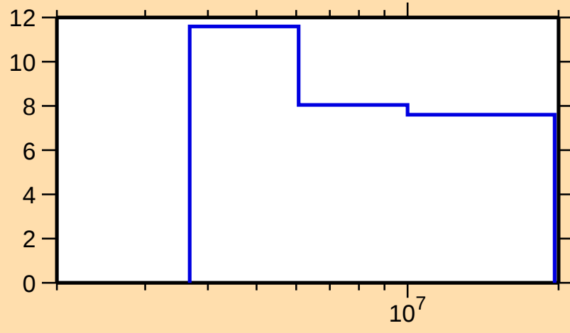
\Delta\sigma/\sigma vs. E for ^{234}\text{Pu}(n,n\text{onel.})
