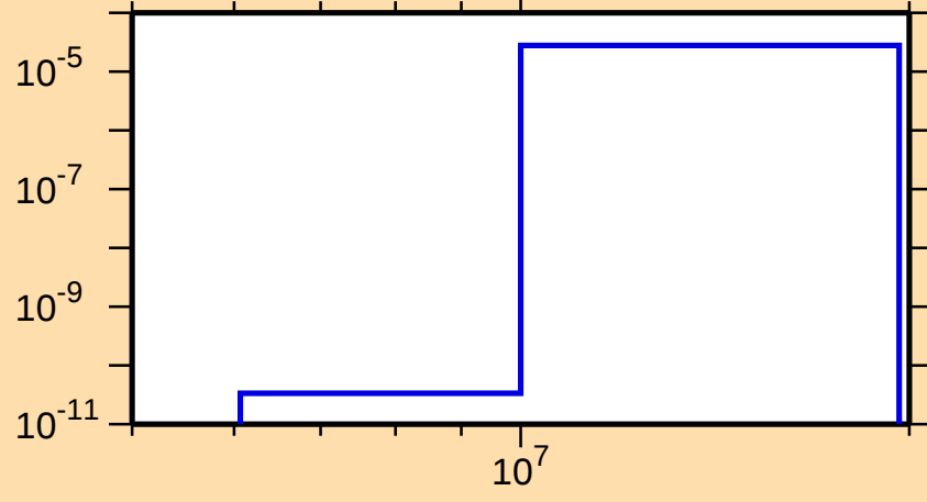
\sigma vs. E for ^{234}\text{Pu}(n,np)
