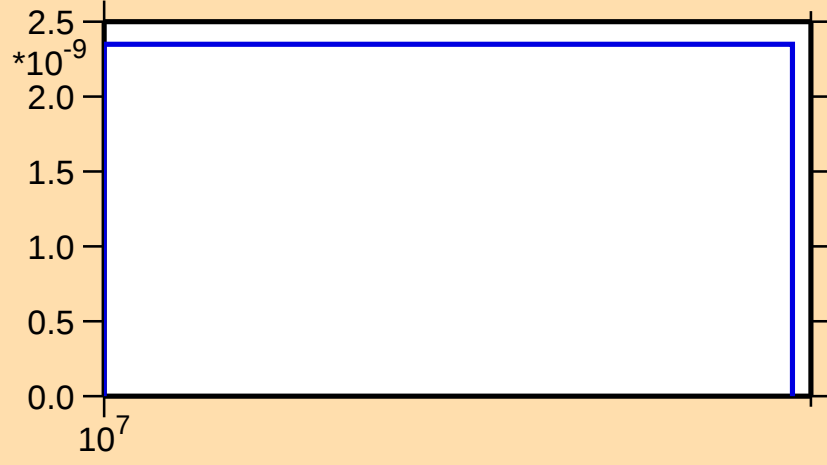
\sigma vs. E for ^{234}\text{Pu}(n,2n\alpha)
