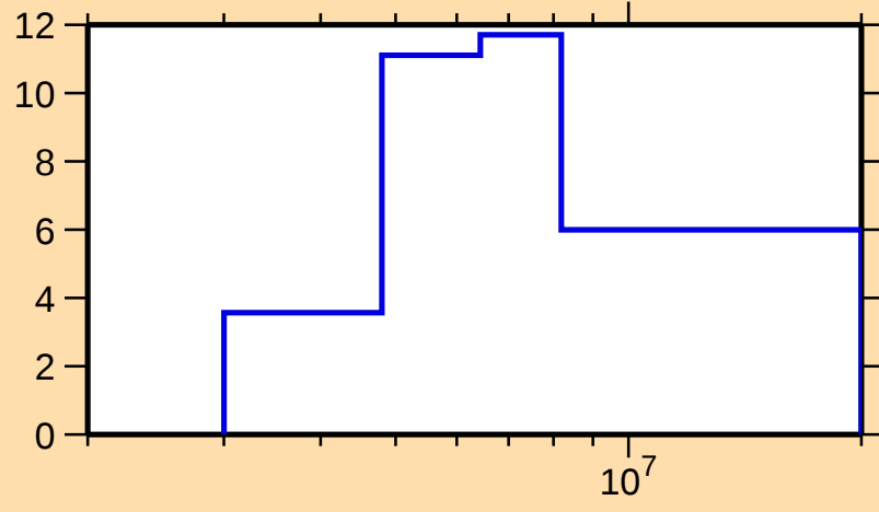
\Delta\sigma/\sigma vs. E for ^{234}\text{Pu}(n,\text{tot.})
