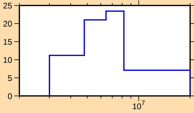
\Delta\sigma/\sigma vs. E for ^{234}\text{Pu}(n,\text{el.})
