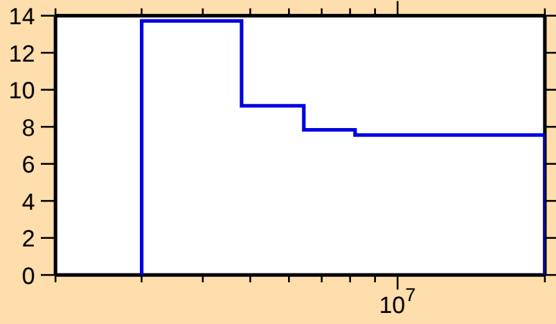
\Delta\sigma/\sigma vs. E for ^{234}\text{Pu}(n,\text{nonel.})
