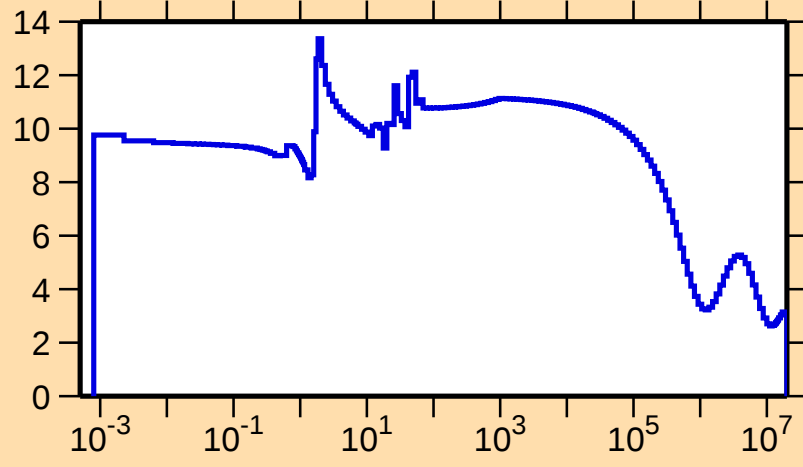
\sigma vs. E for ^{243}\text{Pu}(n,\text{el.})
