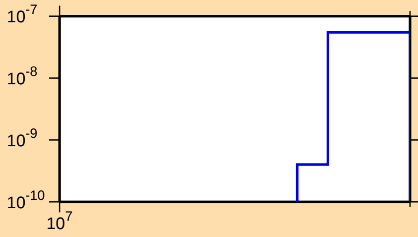
\sigma vs. E for ^{243}\text{Pu}(n,2np)
