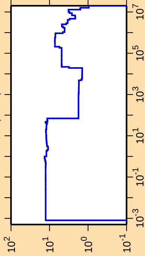
\Delta\sigma/\sigma vs. E for ^{243}\text{Pu}(n,\text{el.})
