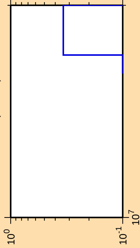
\Delta\sigma/\sigma vs. E for ^{243}\text{Pu}(n,\text{He3})
