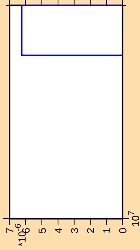
\Delta\sigma/\sigma vs. E for ^{243}\text{Pu} (mt 42)
