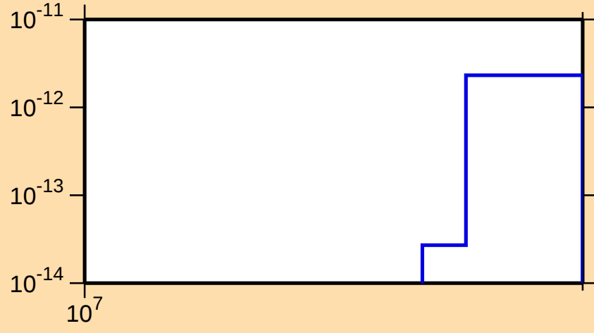
\sigma vs. E for ^{243}\text{Pu}(n,3n\alpha)
