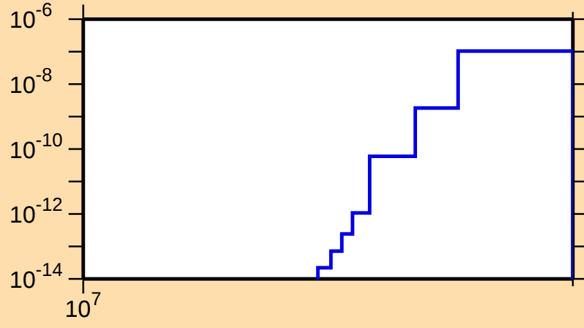
\sigma vs. E for ^{245}\text{Pu}(n,nt)
