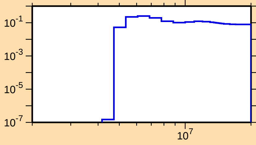
\sigma vs. E for ^{245}\text{Pu}(n,2n)
