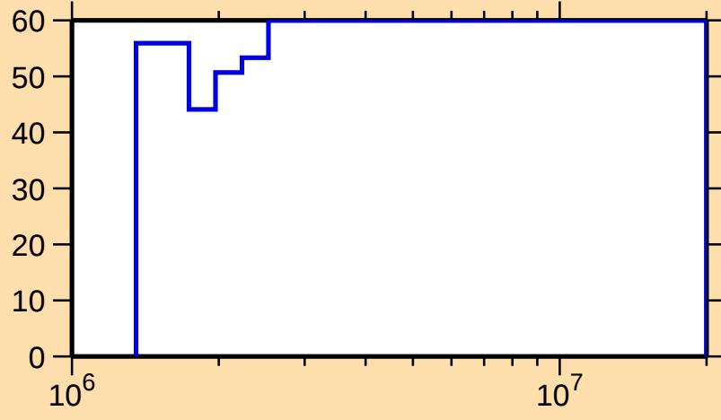
\Delta\sigma/\sigma vs. E for ^{245}\text{Pu}(n,n_1)
