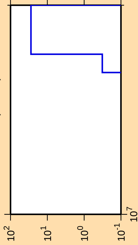
\Delta\sigma/\sigma vs. E for ^{245}\text{Pu}(n,\text{He3})
