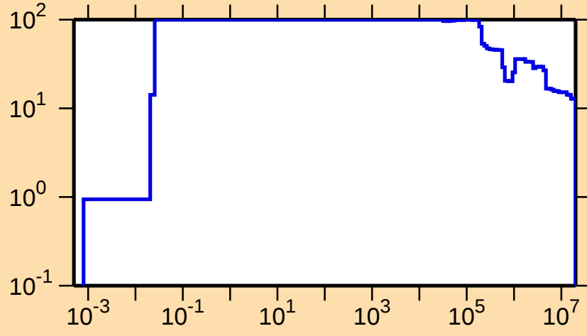
\Delta\sigma/\sigma vs. E for ^{245}\text{Pu}(n,\text{nonel.})
