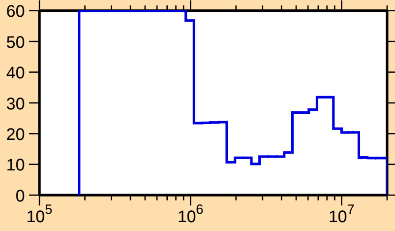
\Delta\sigma/\sigma vs. E for ^{245}\text{Pu}(n,\text{el.})
