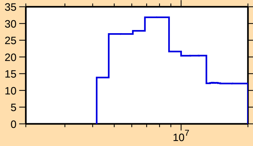
\Delta\sigma/\sigma vs. E for ^{245}\text{Pu}(n,\text{el.})
