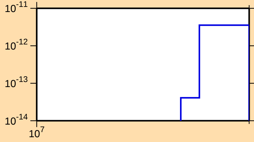
\sigma vs. E for ^{245}\text{Pu}(n,\text{He3})
