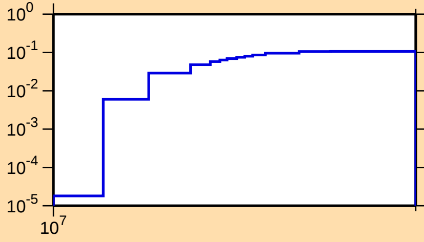
\sigma vs. E for ^{245}\text{Pu}(n,3n)
