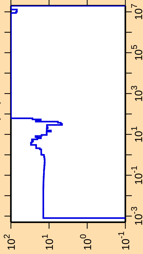
\Delta\sigma/\sigma vs. E for ^{245}\text{Pu}(n,f)
