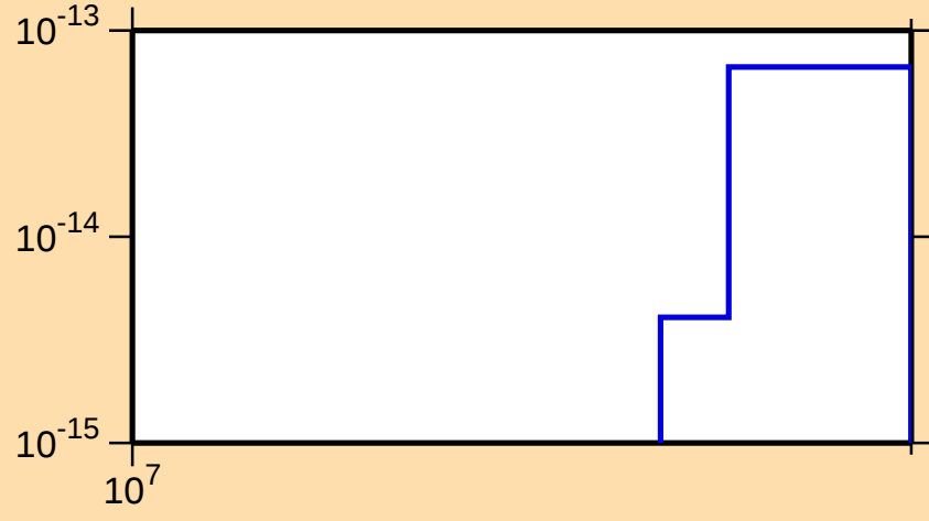
\sigma vs. E for ^{245}\text{Pu}(n,3n\alpha)
